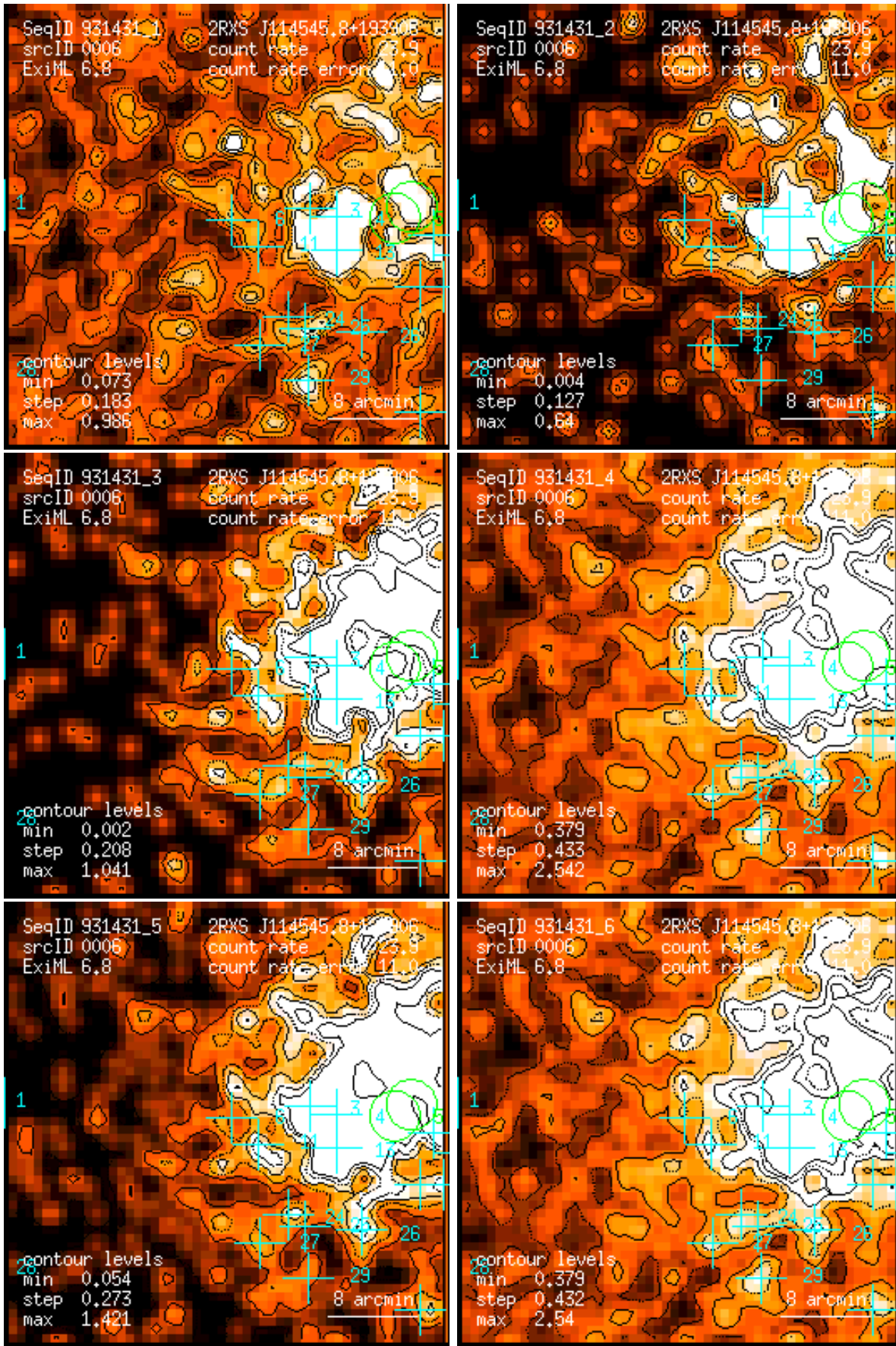
Figure 6: RASS 931431: detection 0006: band rate images, Gaussian filter: (1) PSPC channels 11 – 41, (2) 52 – 90, (3) 91 – 201, (4) 11 – 235, (5) 52 – 201, (6) 11 – 201. Broad band rates in counts/ks. Band rate contour levels in counts/ks/arcmin 2 .
