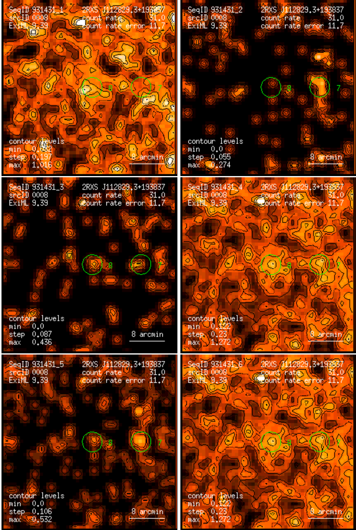
Figure 8: RASS 931431: detection 0008: band rate images, Gaussian filter: (1) PSPC channels 11 – 41, (2) 52 – 90, (3) 91 – 201, (4) 11 – 235, (5) 52 – 201, (6) 11 – 201. Broad band rates in counts/ks. Band rate contour levels in counts/ks/arcmin 2 .
