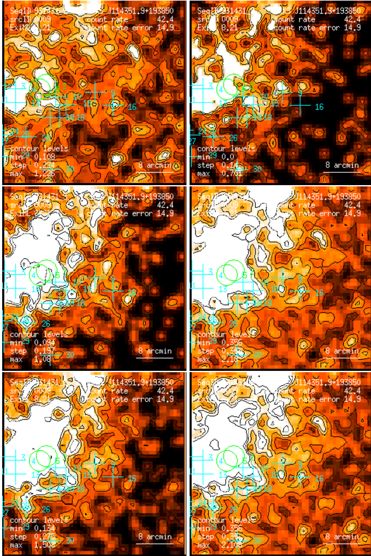
Figure 9: RASS 931431: detection 0009: band rate images, Gaussian filter: (1) PSPC channels 11 – 41, (2) 52 – 90, (3) 91 – 201, (4) 11 – 235, (5) 52 – 201, (6) 11 – 201. Broad band rates in counts/ks. Band rate contour levels in counts/ks/arcmin 2 .
