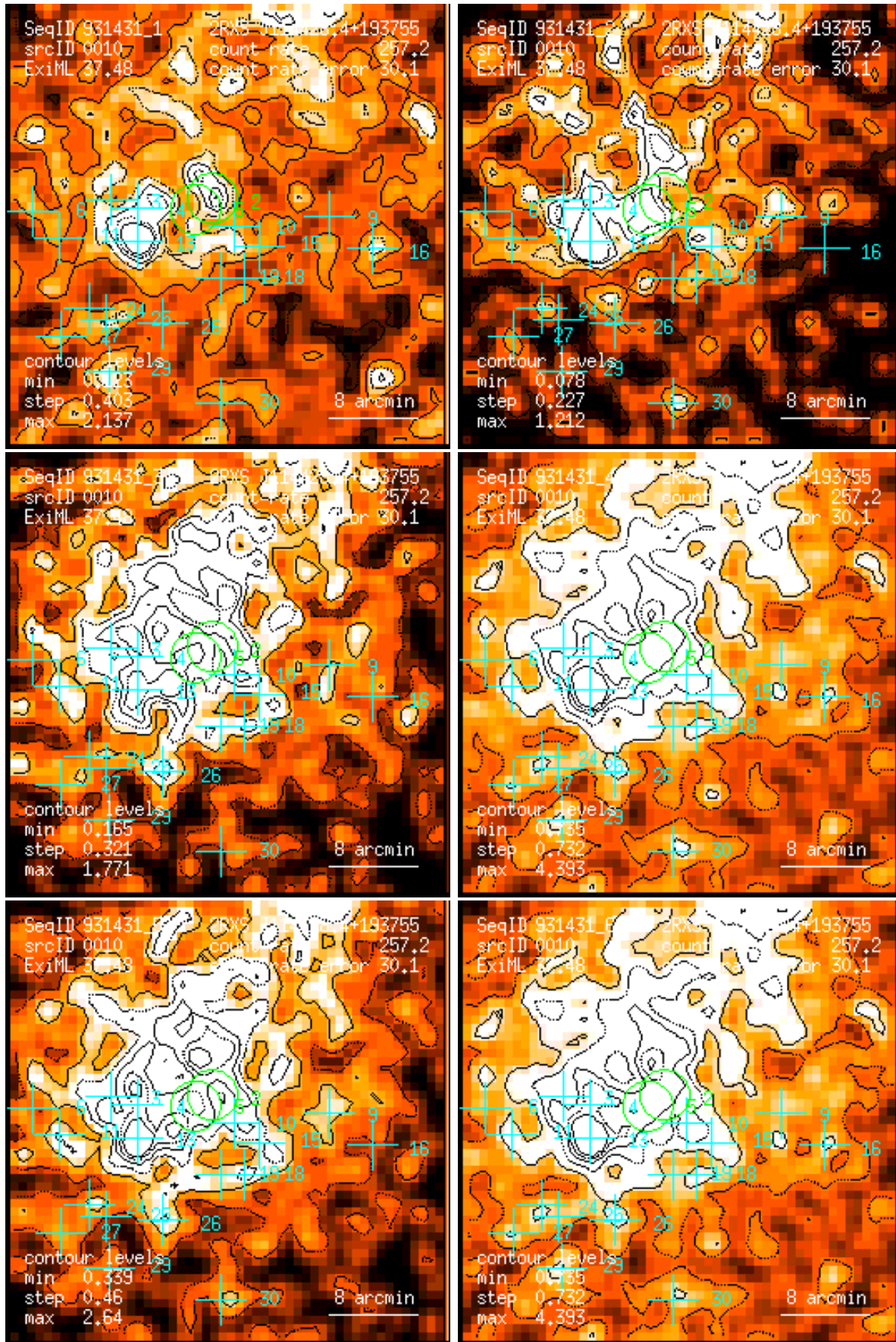
Figure 10: RASS 931431: detection 0010: band rate images, Gaussian filter: (1) PSPC channels 11 – 41, (2) 52 – 90, (3) 91 – 201, (4) 11 – 235, (5) 52 – 201, (6) 11 – 201. Broad band rates in counts/ks. Band rate contour levels in counts/ks/arcmin 2 .
