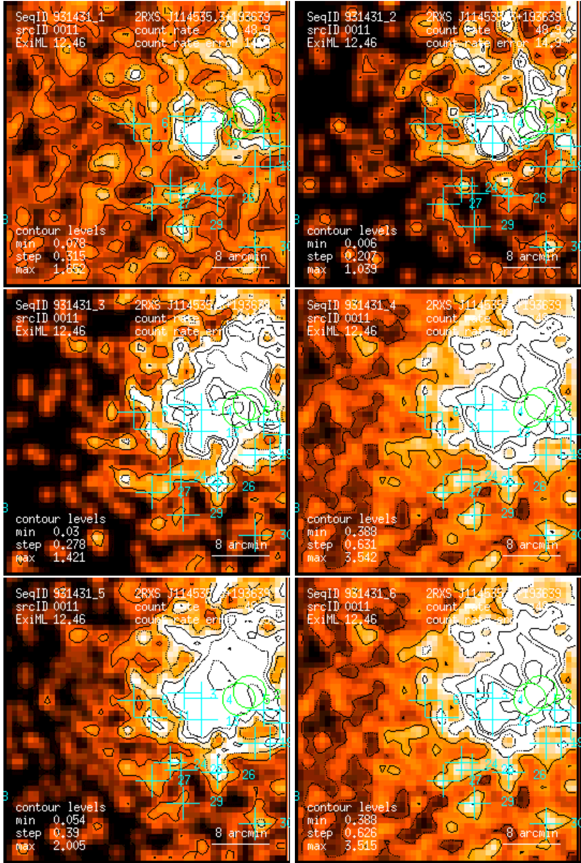
Figure 11: RASS 931431: detection 0011: band rate images, Gaussian filter: (1) PSPC channels 11 – 41, (2) 52 – 90, (3) 91 – 201, (4) 11 – 235, (5) 52 – 201, (6) 11 – 201. Broad band rates in counts/ks. Band rate contour levels in counts/ks/arcmin 2 .
