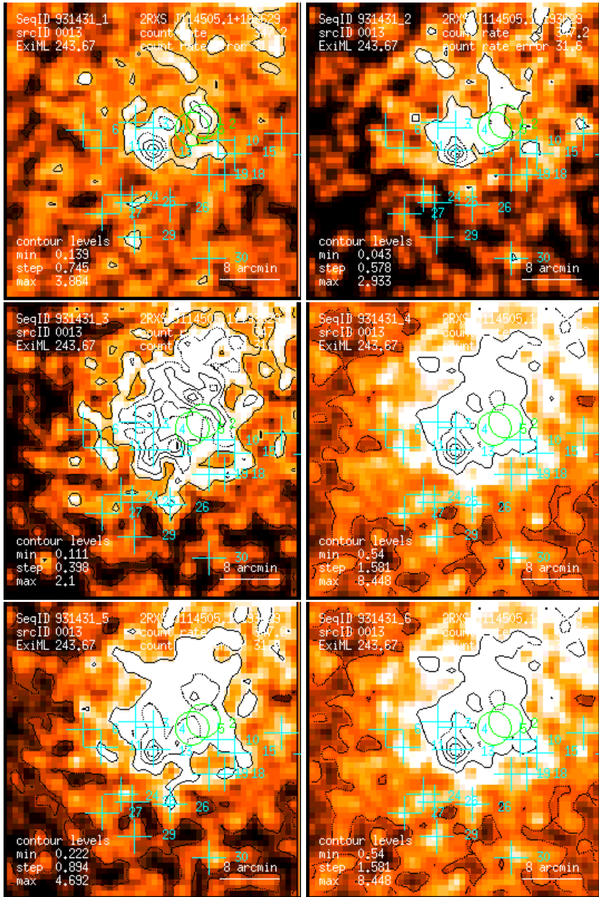
Figure 13: RASS 931431: detection 0013: band rate images, Gaussian filter: (1) PSPC channels 11 – 41, (2) 52 – 90, (3) 91 – 201, (4) 11 – 235, (5) 52 – 201, (6) 11 – 201. Broad band rates in counts/ks. Band rate contour levels in counts/ks/arcmin 2 .
