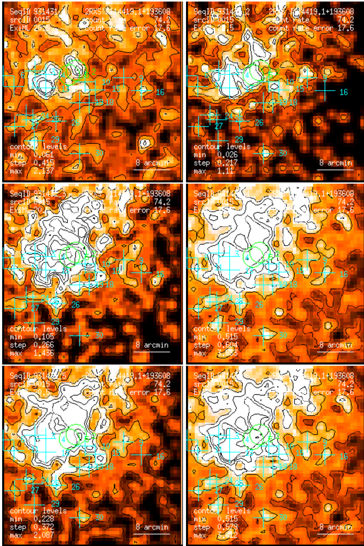
Figure 15: RASS 931431: detection 0015: band rate images, Gaussian filter: (1) PSPC channels 11 – 41, (2) 52 – 90, (3) 91 – 201, (4) 11 – 235, (5) 52 – 201, (6) 11 – 201. Broad band rates in counts/ks. Band rate contour levels in counts/ks/arcmin 2 .
