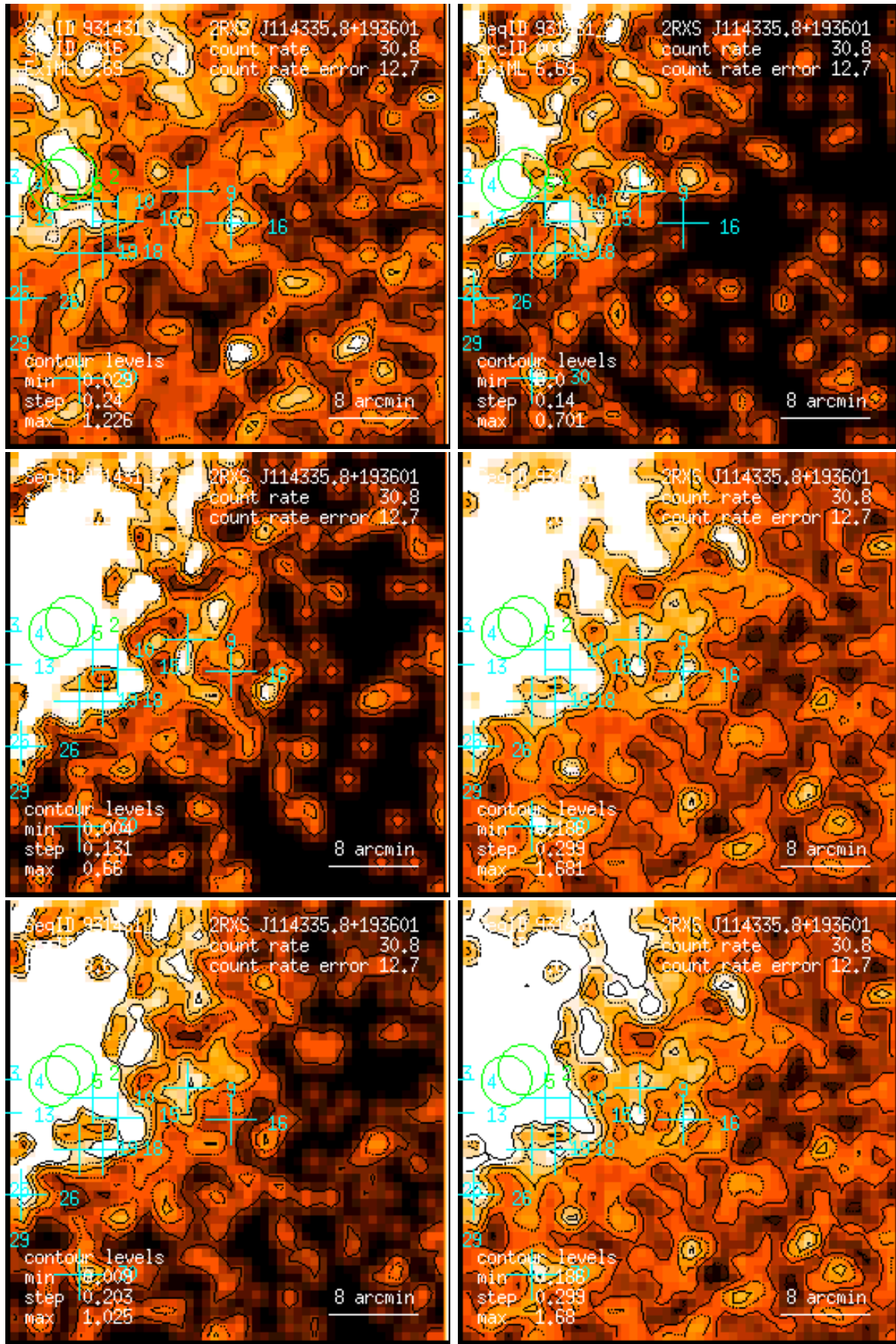
Figure 16: RASS 931431: detection 0016: band rate images, Gaussian filter: (1) PSPC channels 11 – 41, (2) 52 – 90, (3) 91 – 201, (4) 11 – 235, (5) 52 – 201, (6) 11 – 201. Broad band rates in counts/ks. Band rate contour levels in counts/ks/arcmin 2 .
