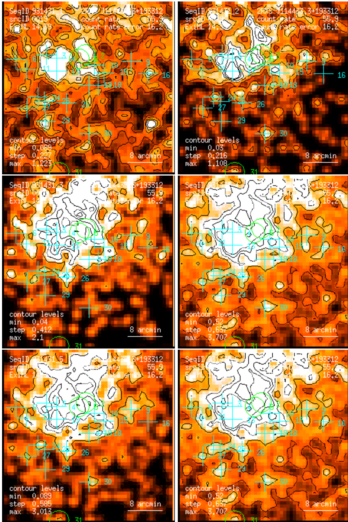
Figure 19: RASS 931431: detection 0019: band rate images, Gaussian filter: (1) PSPC channels 11 – 41, (2) 52 – 90, (3) 91 – 201, (4) 11 – 235, (5) 52 – 201, (6) 11 – 201. Broad band rates in counts/ks. Band rate contour levels in counts/ks/arcmin 2 .
