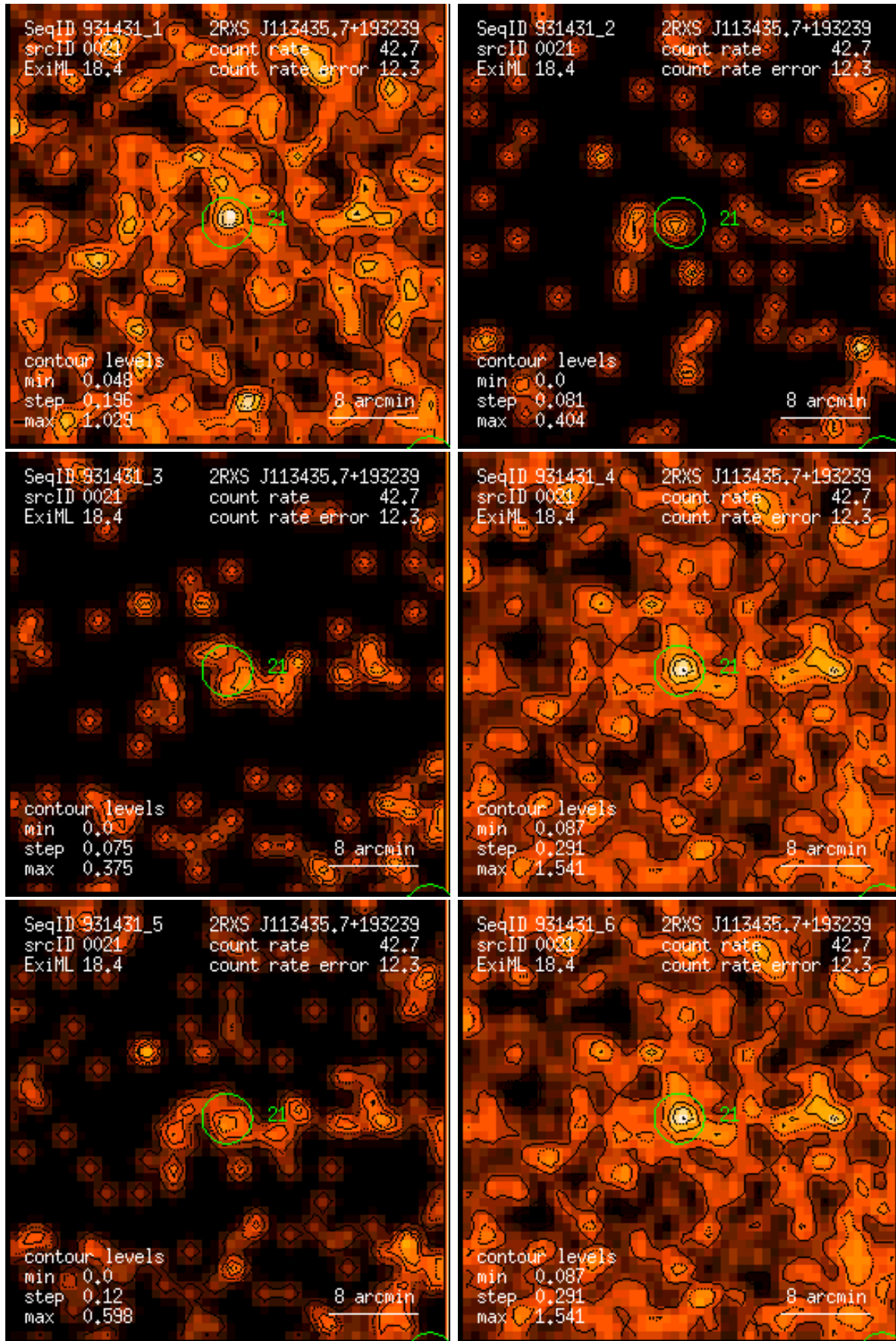
Figure 21: RASS 931431: detection 0021: band rate images, Gaussian filter: (1) PSPC channels 11 – 41, (2) 52 – 90, (3) 91 – 201, (4) 11 – 235, (5) 52 – 201, (6) 11 – 201. Broad band rates in counts/ks. Band rate contour levels in counts/ks/arcmin 2 .
