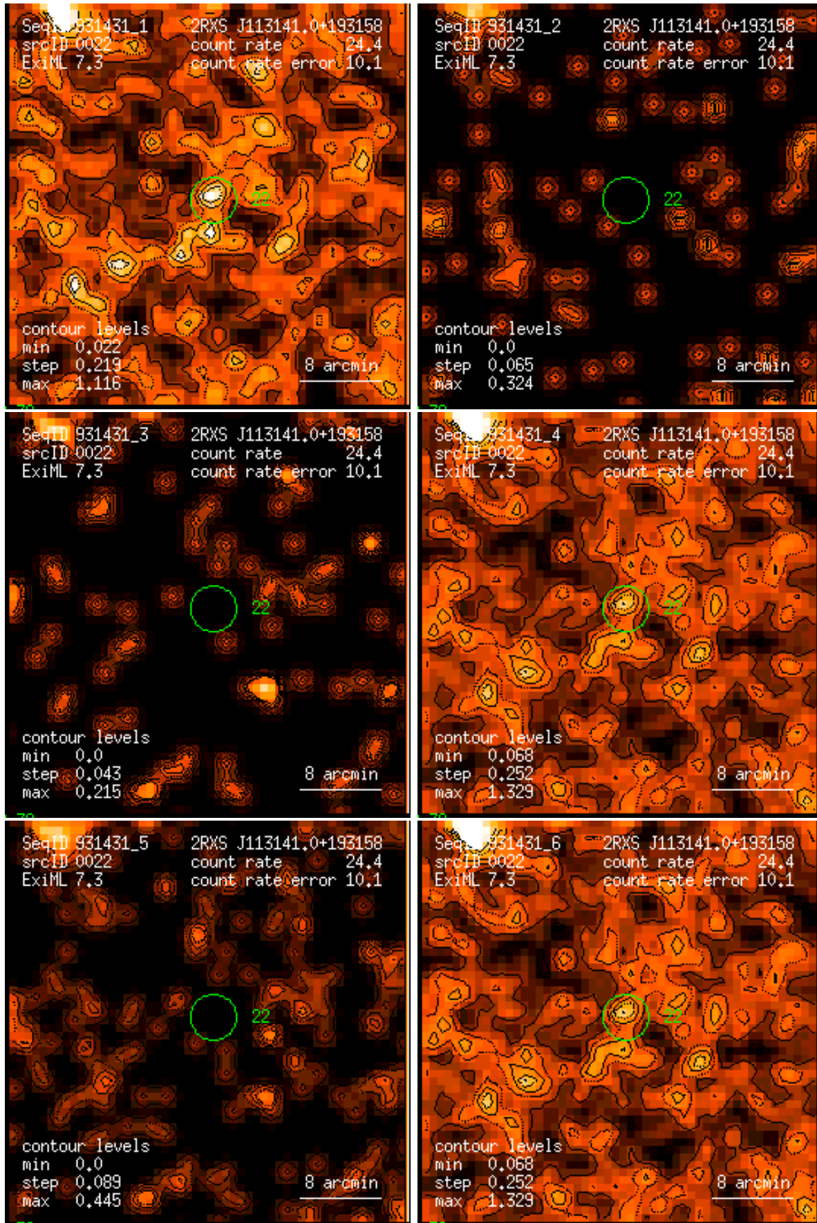
Figure 22: RASS 931431: detection 0022: band rate images, Gaussian filter: (1) PSPC channels 11 – 41, (2) 52 – 90, (3) 91 – 201, (4) 11 – 235, (5) 52 – 201, (6) 11 – 201. Broad band rates in counts/ks. Band rate contour levels in counts/ks/arcmin 2 .
