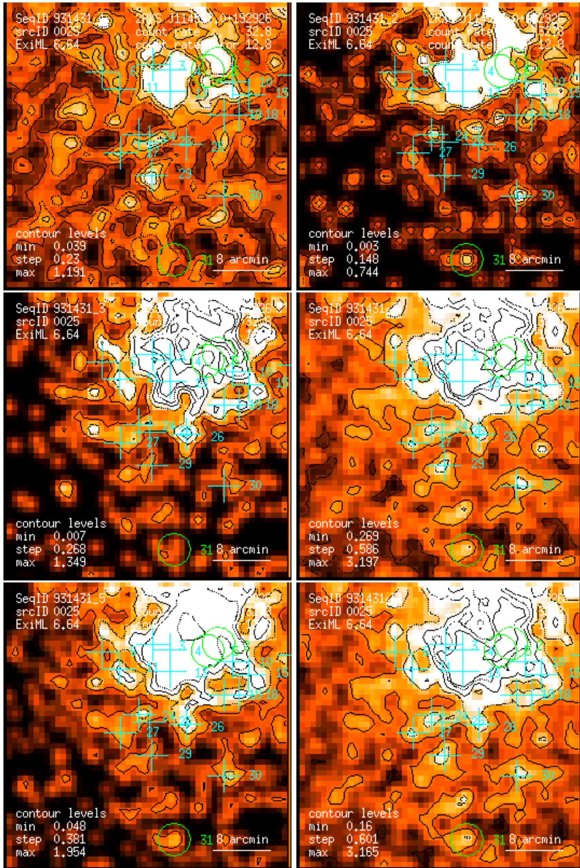
Figure 25: RASS 931431: detection 0025: band rate images, Gaussian filter: (1) PSPC channels 11 – 41, (2) 52 – 90, (3) 91 – 201, (4) 11 – 235, (5) 52 – 201, (6) 11 – 201. Broad band rates in counts/ks. Band rate contour levels in counts/ks/arcmin 2 .
