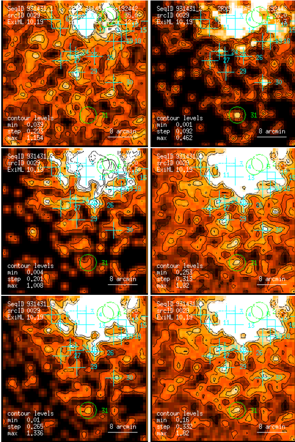
Figure 29: RASS 931431: detection 0029: band rate images, Gaussian filter: (1) PSPC channels 11 – 41, (2) 52 – 90, (3) 91 – 201, (4) 11 – 235, (5) 52 – 201, (6) 11 – 201. Broad band rates in counts/ks. Band rate contour levels in counts/ks/arcmin 2 .
