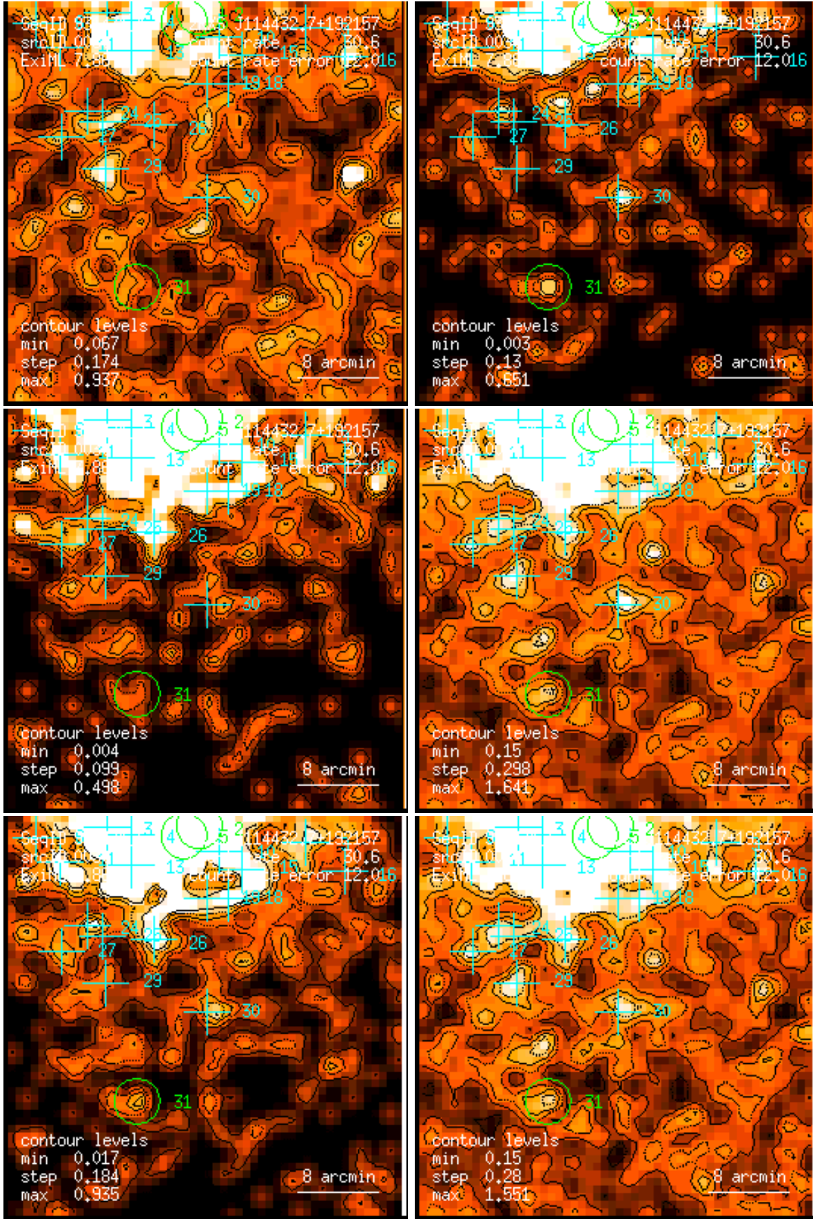
Figure 30: RASS 931431: detection 0030: band rate images, Gaussian filter: (1) PSPC channels 11 – 41, (2) 52 – 90, (3) 91 – 201, (4) 11 – 235, (5) 52 – 201, (6) 11 – 201. Broad band rates in counts/ks. Band rate contour levels in counts/ks/arcmin 2 .
