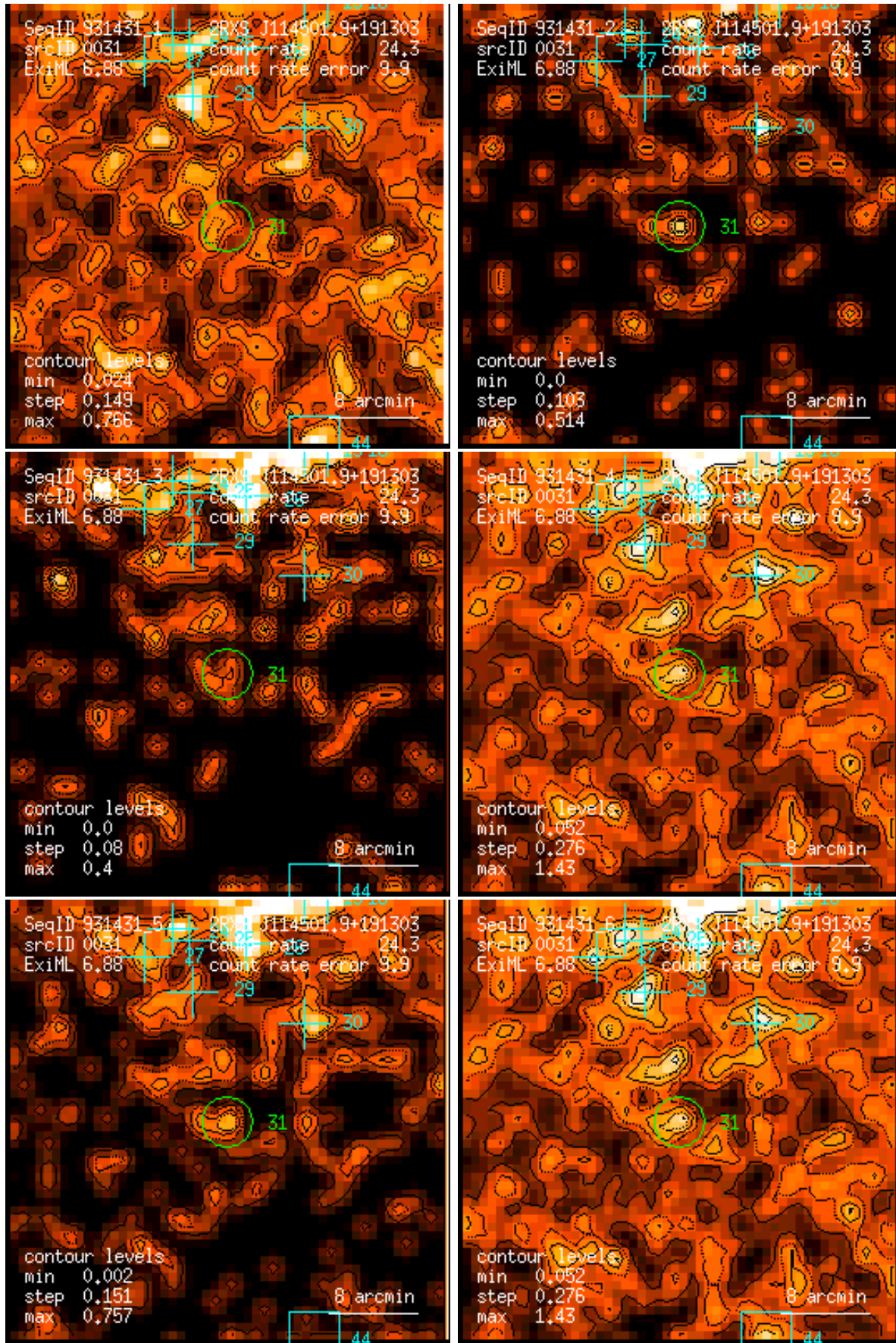
Figure 31: RASS 931431: detection 0031: band rate images, Gaussian filter: (1) PSPC channels 11 – 41, (2) 52 – 90, (3) 91 – 201, (4) 11 – 235, (5) 52 – 201, (6) 11 – 201. Broad band rates in counts/ks. Band rate contour levels in counts/ks/arcmin 2 .
