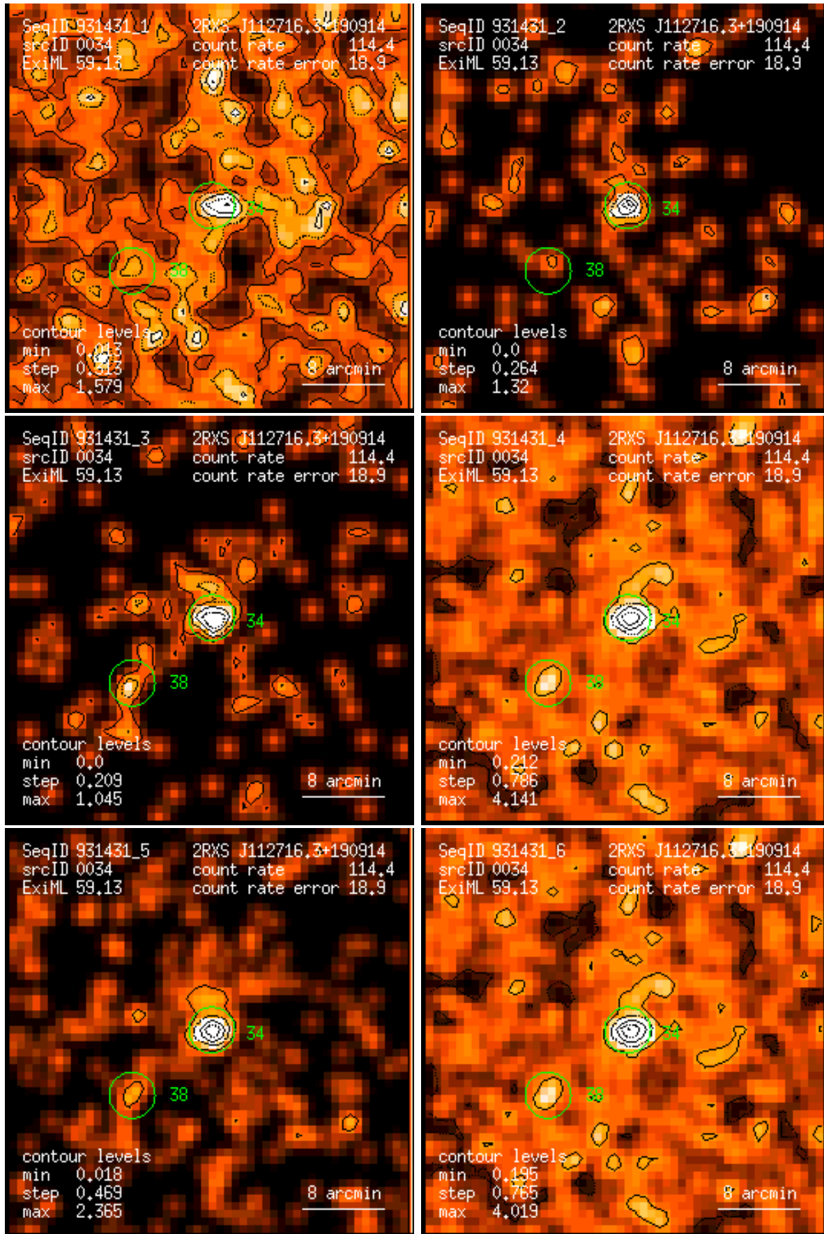
Figure 34: RASS 931431: detection 0034: band rate images, Gaussian filter: (1) PSPC channels 11 – 41, (2) 52 – 90, (3) 91 – 201, (4) 11 – 235, (5) 52 – 201, (6) 11 – 201. Broad band rates in counts/ks. Band rate contour levels in counts/ks/arcmin 2 .
