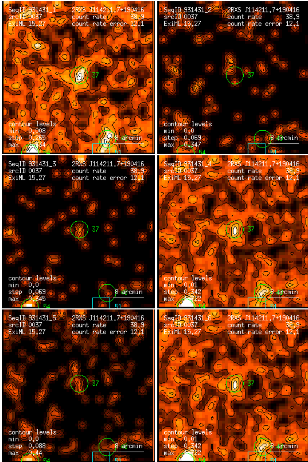
Figure 37: RASS 931431: detection 0037: band rate images, Gaussian filter: (1) PSPC channels 11 – 41, (2) 52 – 90, (3) 91 – 201, (4) 11 – 235, (5) 52 – 201, (6) 11 – 201. Broad band rates in counts/ks. Band rate contour levels in counts/ks/arcmin 2 .
