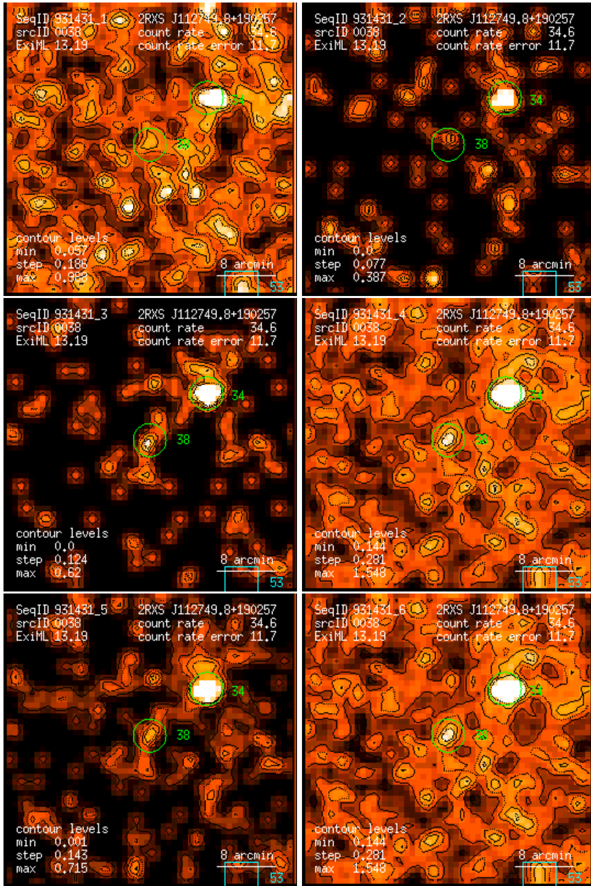
Figure 38: RASS 931431: detection 0038: band rate images, Gaussian filter: (1) PSPC channels 11 – 41, (2) 52 – 90, (3) 91 – 201, (4) 11 – 235, (5) 52 – 201, (6) 11 – 201. Broad band rates in counts/ks. Band rate contour levels in counts/ks/arcmin 2 .
