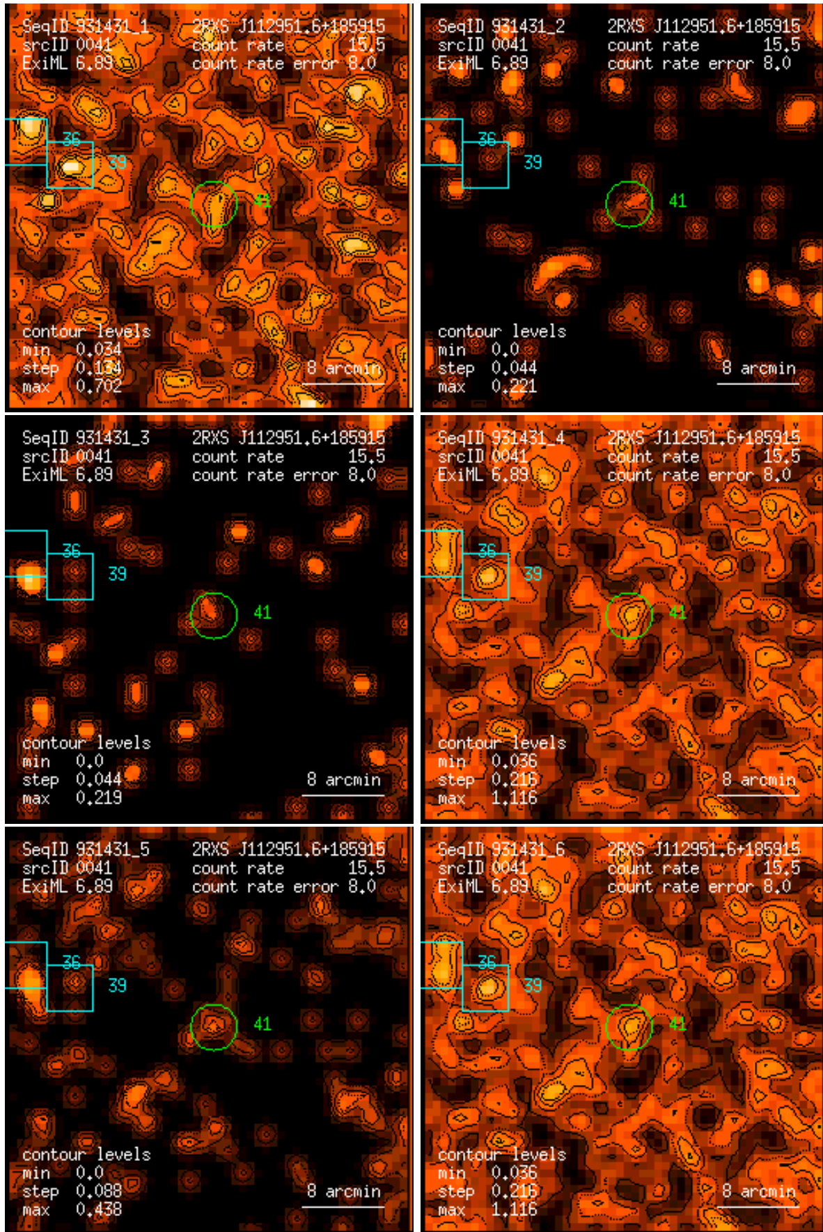
Figure 41: RASS 931431: detection 0041: band rate images, Gaussian filter: (1) PSPC channels 11 – 41, (2) 52 – 90, (3) 91 – 201, (4) 11 – 235, (5) 52 – 201, (6) 11 – 201. Broad band rates in counts/ks. Band rate contour levels in counts/ks/arcmin 2 .
