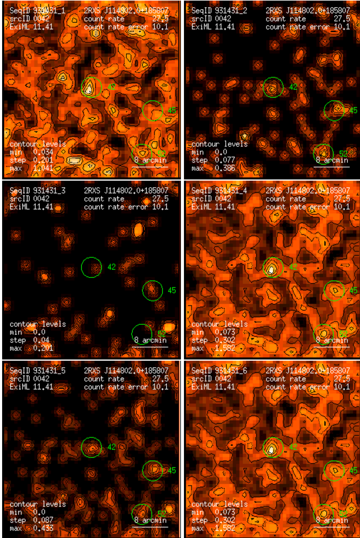
Figure 42: RASS 931431: detection 0042: band rate images, Gaussian filter: (1) PSPC channels 11 – 41, (2) 52 – 90, (3) 91 – 201, (4) 11 – 235, (5) 52 – 201, (6) 11 – 201. Broad band rates in counts/ks. Band rate contour levels in counts/ks/arcmin 2 .
