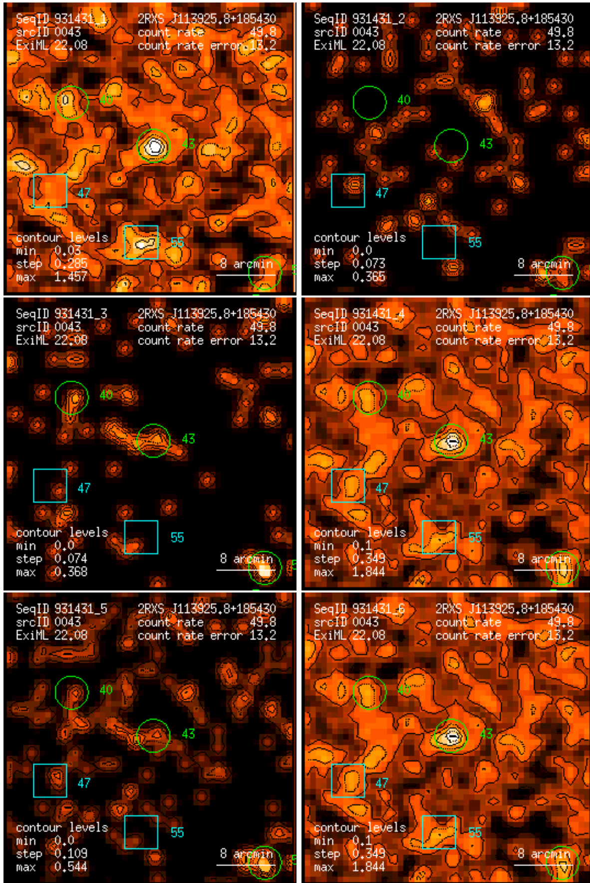
Figure 43: RASS 931431: detection 0043: band rate images, Gaussian filter: (1) PSPC channels 11 – 41, (2) 52 – 90, (3) 91 – 201, (4) 11 – 235, (5) 52 – 201, (6) 11 – 201. Broad band rates in counts/ks. Band rate contour levels in counts/ks/arcmin 2 .
