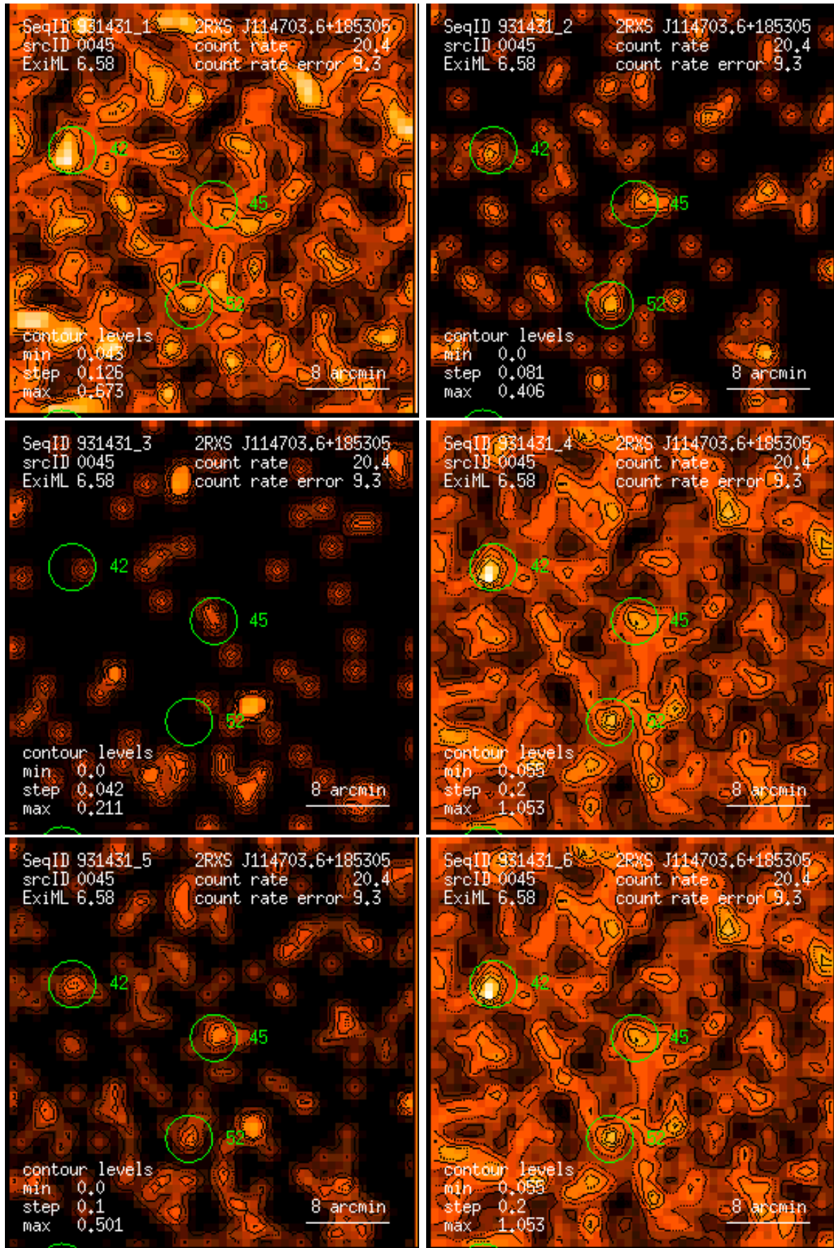
Figure 45: RASS 931431: detection 0045: band rate images, Gaussian filter: (1) PSPC channels 11 – 41, (2) 52 – 90, (3) 91 – 201, (4) 11 – 235, (5) 52 – 201, (6) 11 – 201. Broad band rates in counts/ks. Band rate contour levels in counts/ks/arcmin 2 .
