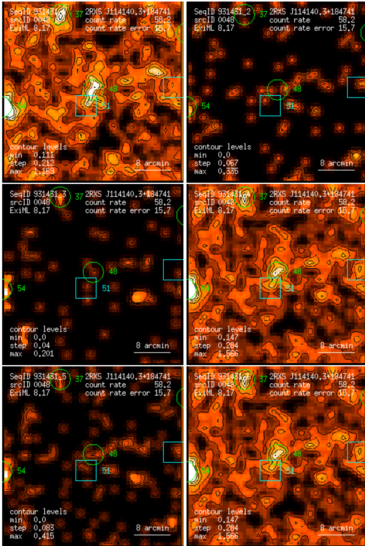
Figure 48: RASS 931431: detection 0048: band rate images, Gaussian filter: (1) PSPC channels 11 – 41, (2) 52 – 90, (3) 91 – 201, (4) 11 – 235, (5) 52 – 201, (6) 11 – 201. Broad band rates in counts/ks. Band rate contour levels in counts/ks/arcmin 2 .
