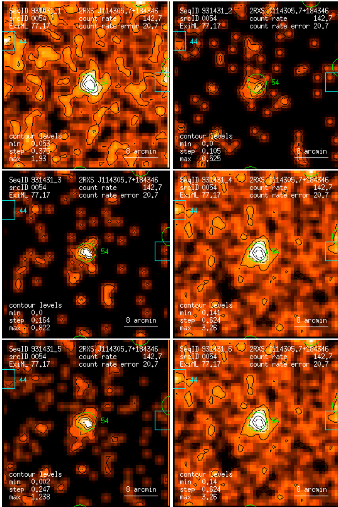
Figure 54: RASS 931431: detection 0054: band rate images, Gaussian filter: (1) PSPC channels 11 – 41, (2) 52 – 90, (3) 91 – 201, (4) 11 – 235, (5) 52 – 201, (6) 11 – 201. Broad band rates in counts/ks. Band rate contour levels in counts/ks/arcmin 2 .
