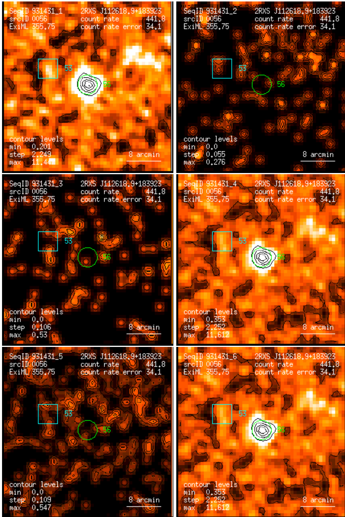
Figure 56: RASS 931431: detection 0056: band rate images, Gaussian filter: (1) PSPC channels 11 – 41, (2) 52 – 90, (3) 91 – 201, (4) 11 – 235, (5) 52 – 201, (6) 11 – 201. Broad band rates in counts/ks. Band rate contour levels in counts/ks/arcmin 2 .
