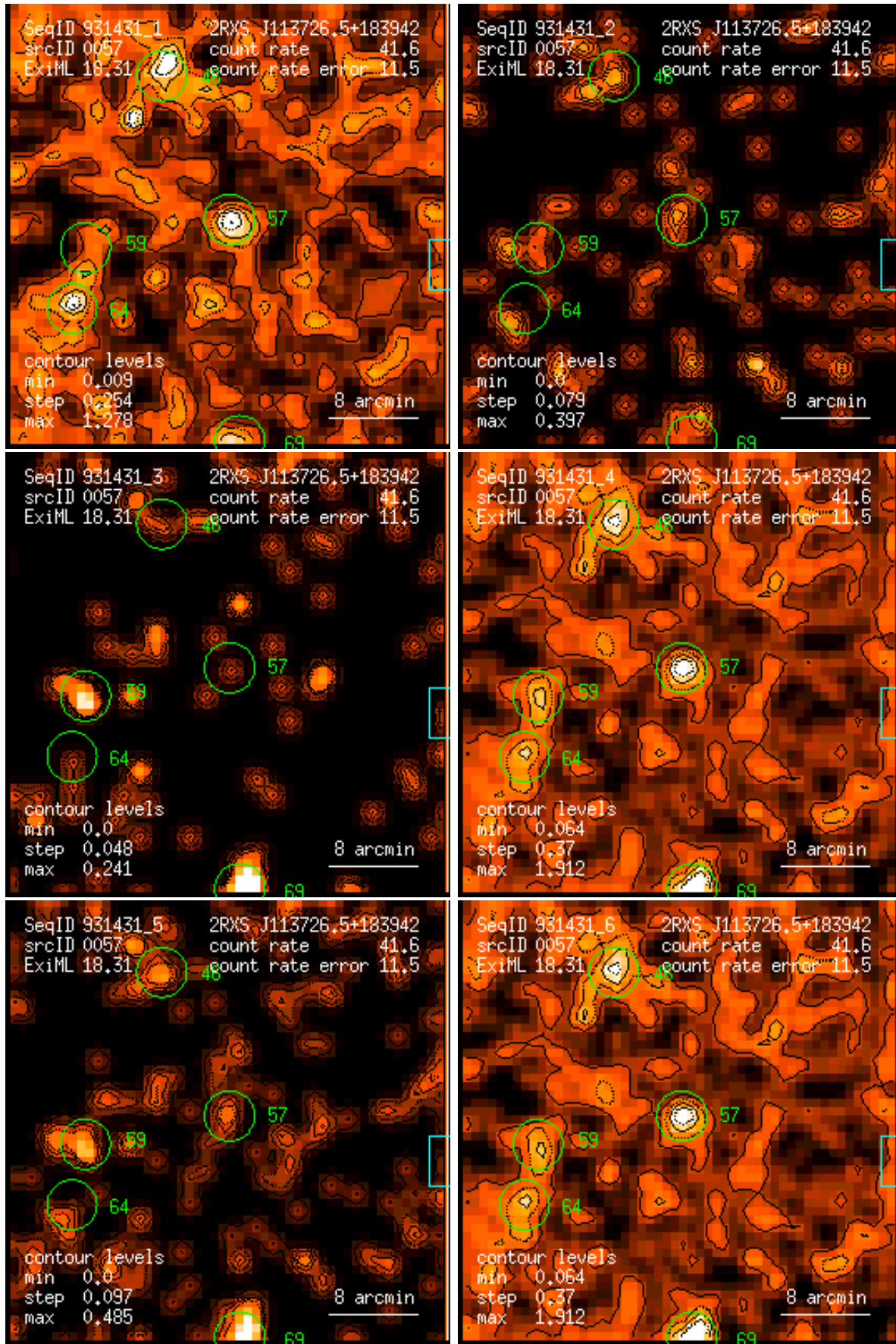
Figure 57: RASS 931431: detection 0057: band rate images, Gaussian filter: (1) PSPC channels 11 – 41, (2) 52 – 90, (3) 91 – 201, (4) 11 – 235, (5) 52 – 201, (6) 11 – 201. Broad band rates in counts/ks. Band rate contour levels in counts/ks/arcmin 2 .
