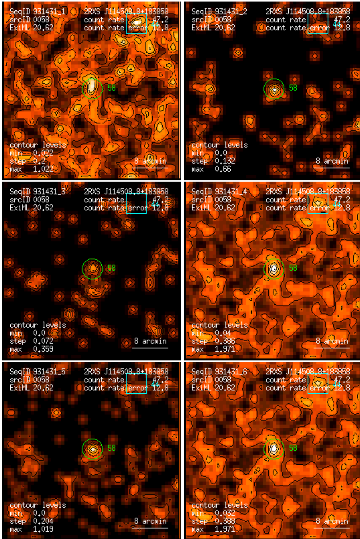
Figure 58: RASS 931431: detection 0058: band rate images, Gaussian filter: (1) PSPC channels 11 – 41, (2) 52 – 90, (3) 91 – 201, (4) 11 – 235, (5) 52 – 201, (6) 11 – 201. Broad band rates in counts/ks. Band rate contour levels in counts/ks/arcmin 2 .
