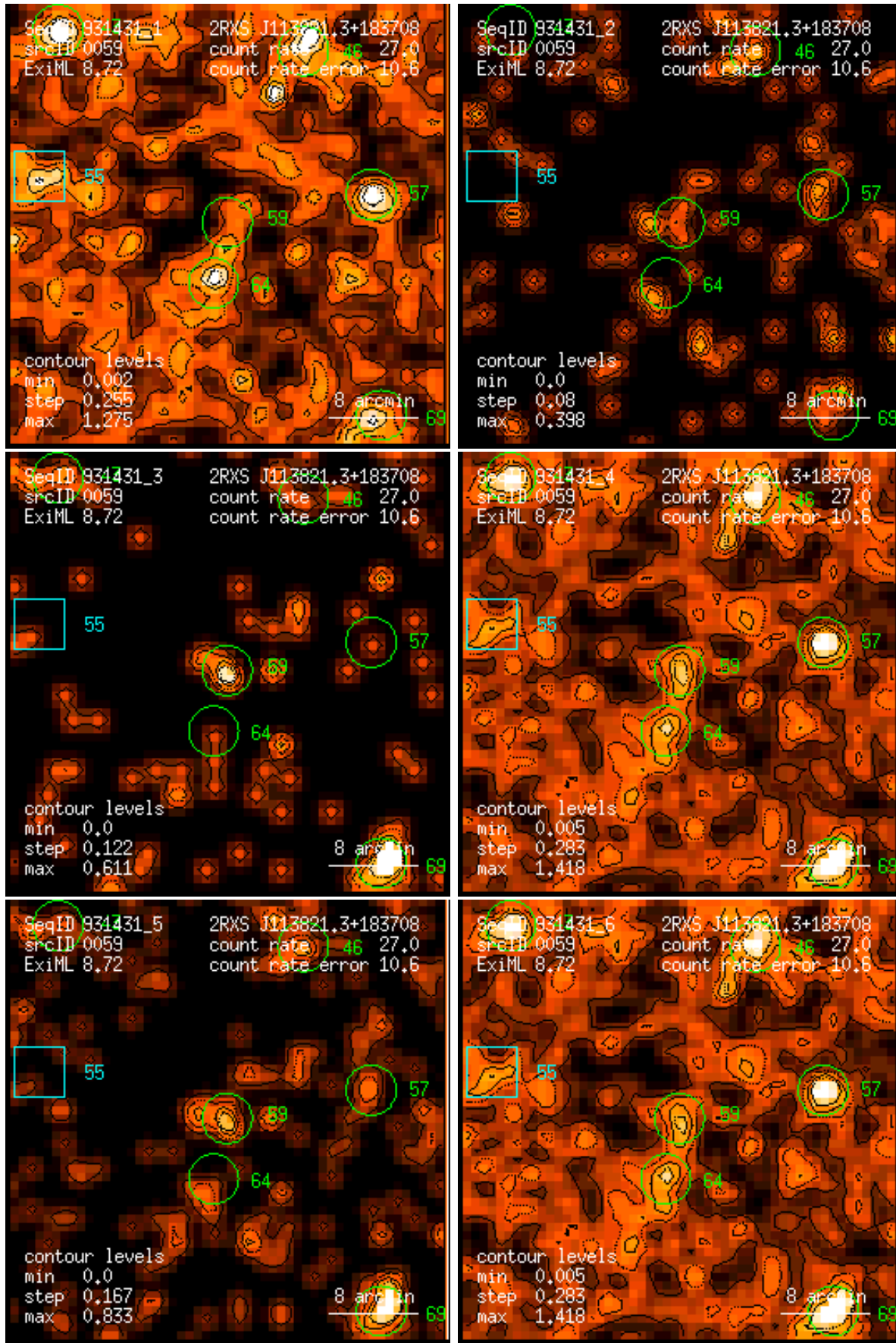
Figure 59: RASS 931431: detection 0059: band rate images, Gaussian filter: (1) PSPC channels 11 – 41, (2) 52 – 90, (3) 91 – 201, (4) 11 – 235, (5) 52 – 201, (6) 11 – 201. Broad band rates in counts/ks. Band rate contour levels in counts/ks/arcmin 2 .
