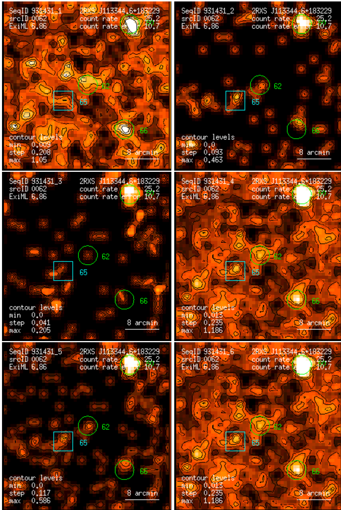
Figure 62: RASS 931431: detection 0062: band rate images, Gaussian filter: (1) PSPC channels 11 – 41, (2) 52 – 90, (3) 91 – 201, (4) 11 – 235, (5) 52 – 201, (6) 11 – 201. Broad band rates in counts/ks. Band rate contour levels in counts/ks/arcmin 2 .
