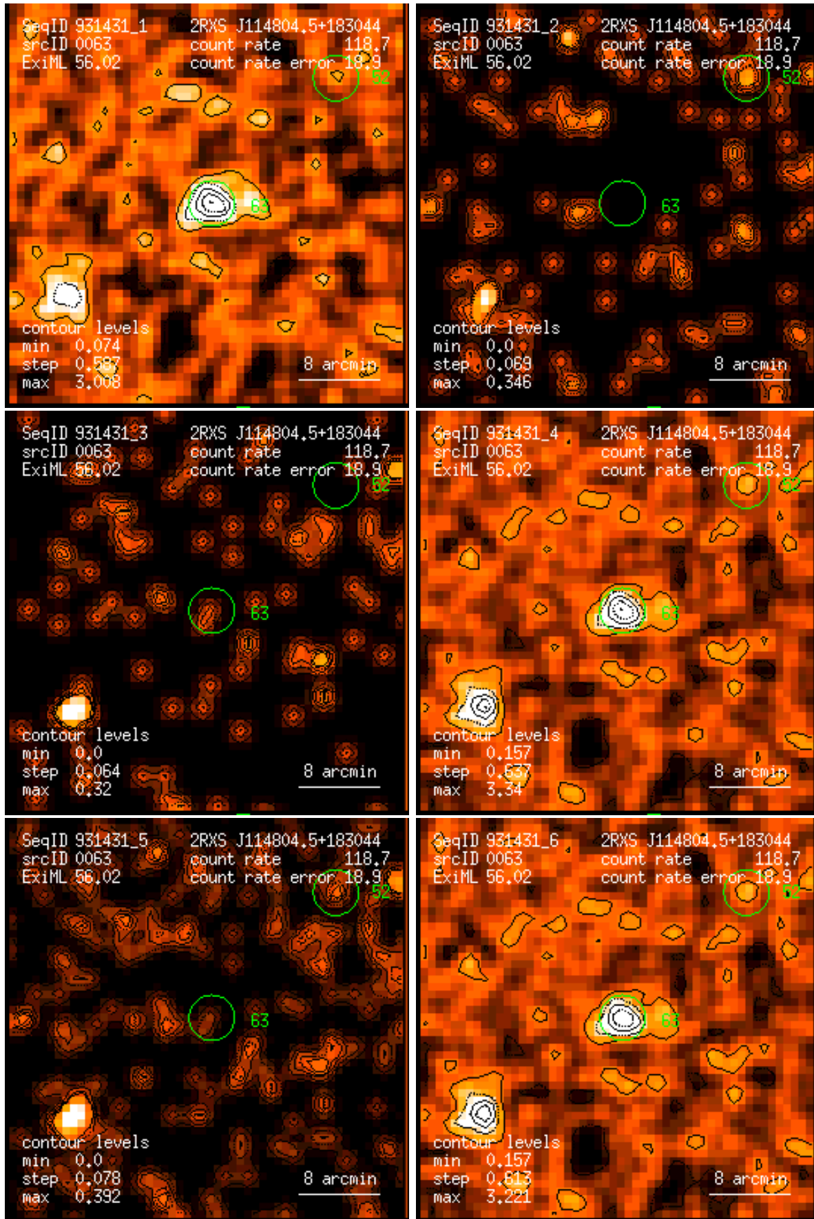
Figure 63: RASS 931431: detection 0063: band rate images, Gaussian filter: (1) PSPC channels 11 – 41, (2) 52 – 90, (3) 91 – 201, (4) 11 – 235, (5) 52 – 201, (6) 11 – 201. Broad band rates in counts/ks. Band rate contour levels in counts/ks/arcmin 2 .
