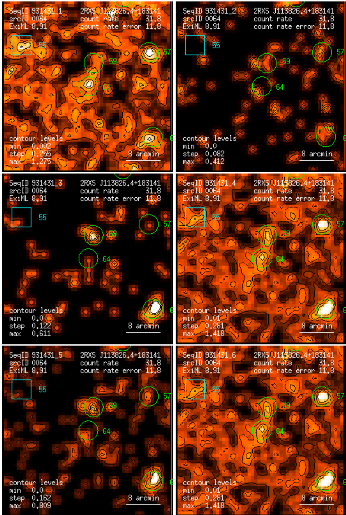
Figure 64: RASS 931431: detection 0064: band rate images, Gaussian filter: (1) PSPC channels 11 – 41, (2) 52 – 90, (3) 91 – 201, (4) 11 – 235, (5) 52 – 201, (6) 11 – 201. Broad band rates in counts/ks. Band rate contour levels in counts/ks/arcmin 2 .
