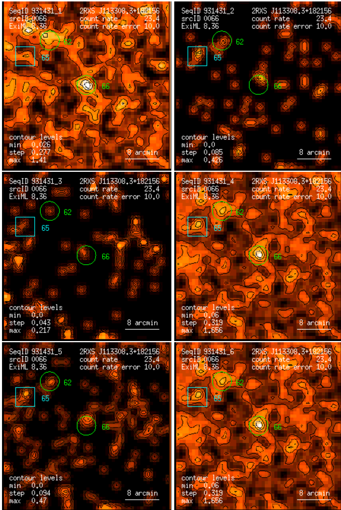
Figure 66: RASS 931431: detection 0066: band rate images, Gaussian filter: (1) PSPC channels 11 – 41, (2) 52 – 90, (3) 91 – 201, (4) 11 – 235, (5) 52 – 201, (6) 11 – 201. Broad band rates in counts/ks. Band rate contour levels in counts/ks/arcmin 2 .
