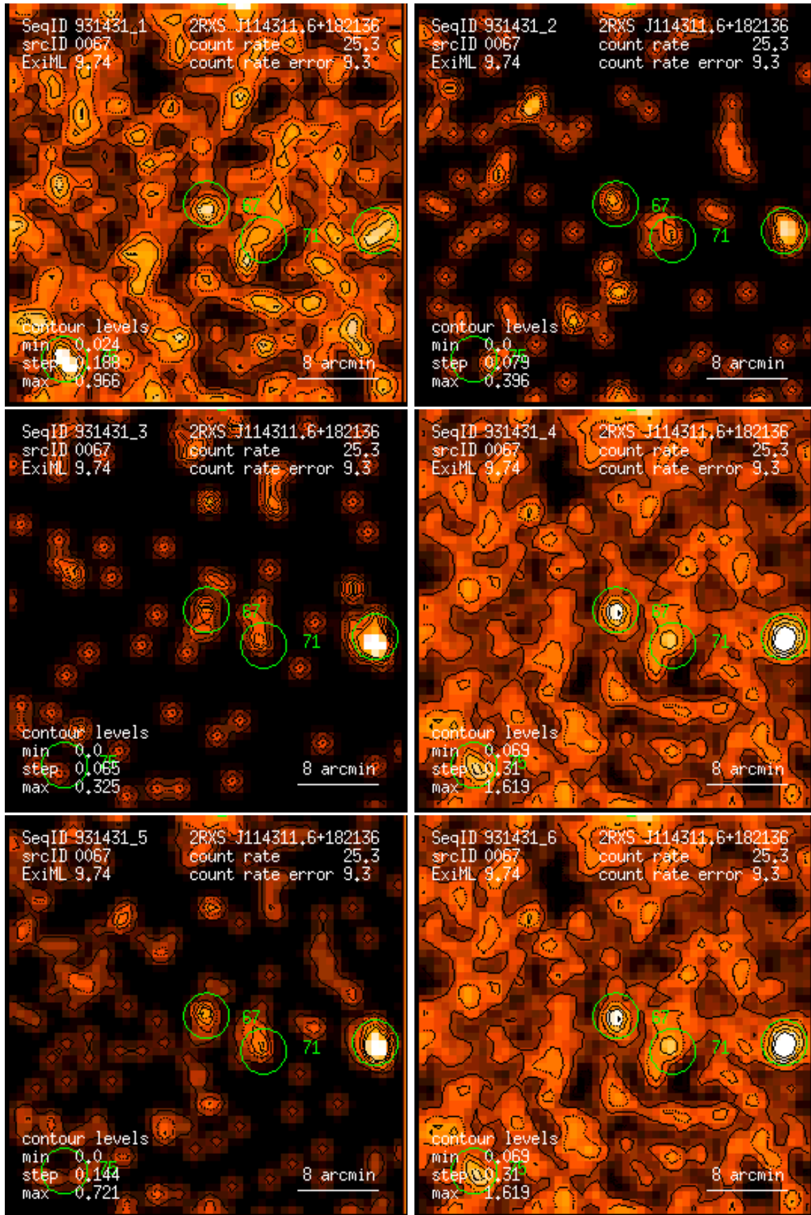
Figure 67: RASS 931431: detection 0067: band rate images, Gaussian filter: (1) PSPC channels 11 – 41, (2) 52 – 90, (3) 91 – 201, (4) 11 – 235, (5) 52 – 201, (6) 11 – 201. Broad band rates in counts/ks. Band rate contour levels in counts/ks/arcmin 2 .
