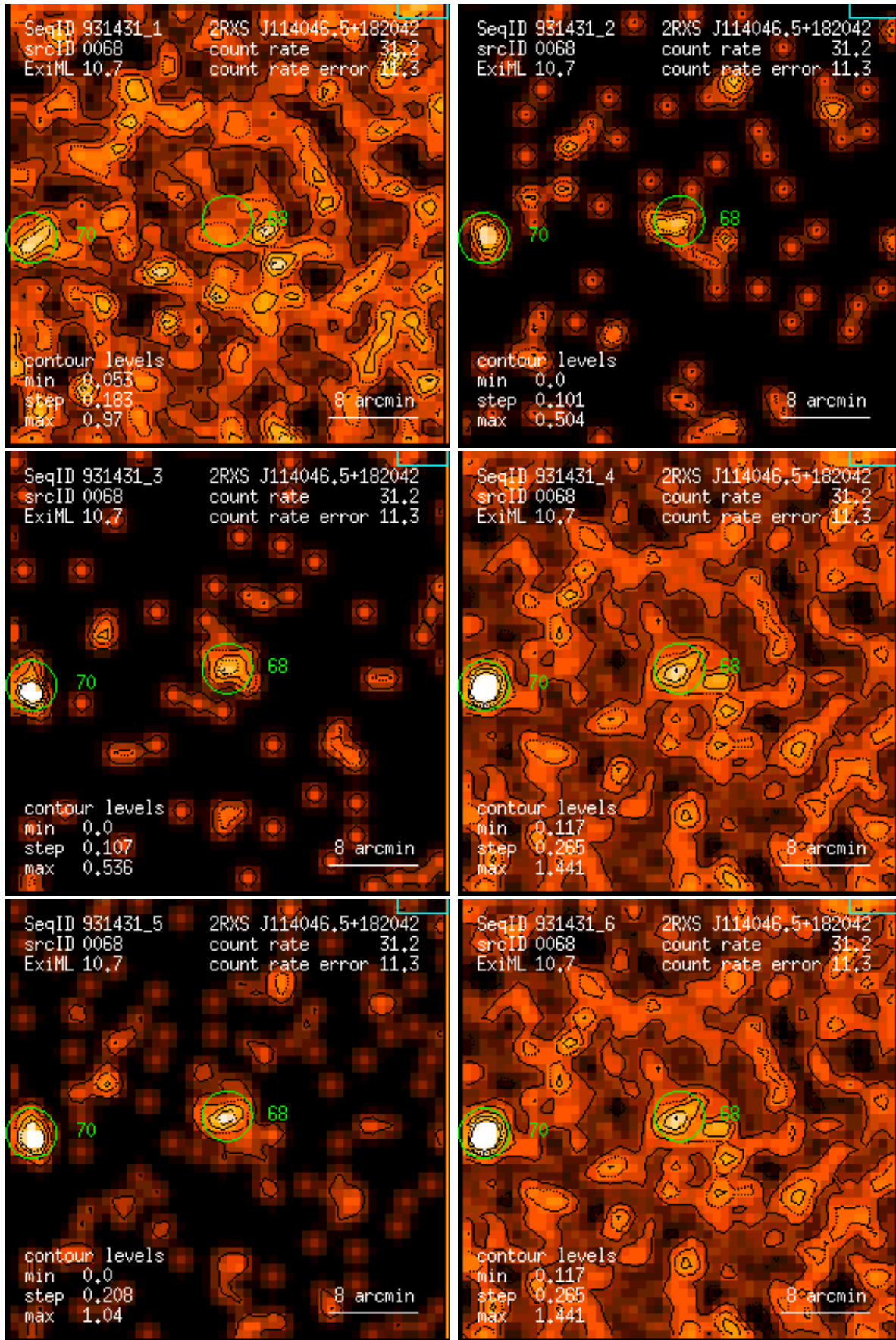
Figure 68: RASS 931431: detection 0068: band rate images, Gaussian filter: (1) PSPC channels 11 – 41, (2) 52 – 90, (3) 91 – 201, (4) 11 – 235, (5) 52 – 201, (6) 11 – 201. Broad band rates in counts/ks. Band rate contour levels in counts/ks/arcmin 2 .
