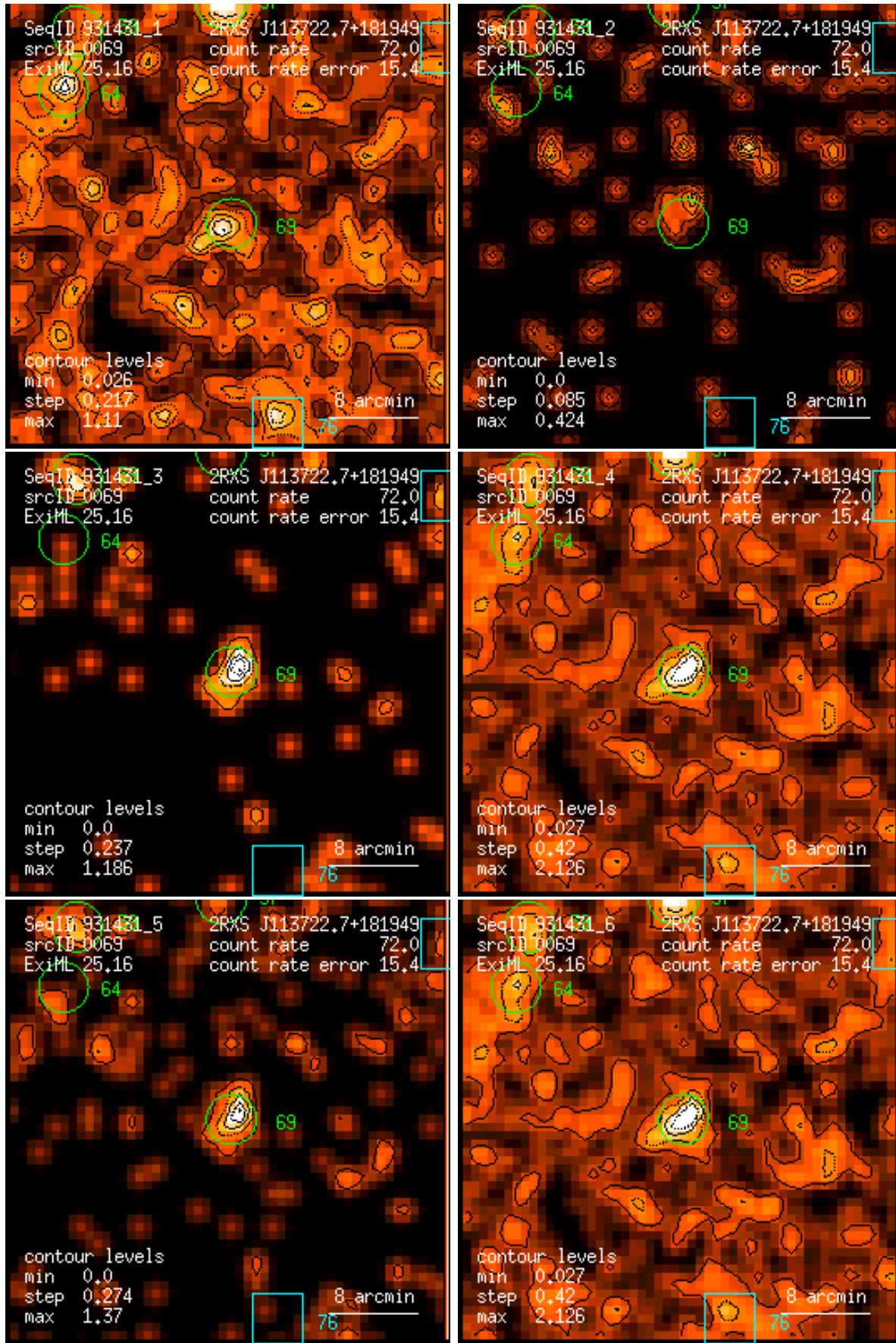
Figure 69: RASS 931431: detection 0069: band rate images, Gaussian filter: (1) PSPC channels 11 – 41, (2) 52 – 90, (3) 91 – 201, (4) 11 – 235, (5) 52 – 201, (6) 11 – 201. Broad band rates in counts/ks. Band rate contour levels in counts/ks/arcmin 2 .
