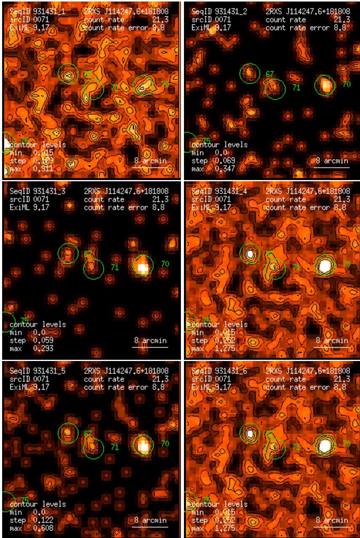
Figure 71: RASS 931431: detection 0071: band rate images, Gaussian filter: (1) PSPC channels 11 – 41, (2) 52 – 90, (3) 91 – 201, (4) 11 – 235, (5) 52 – 201, (6) 11 – 201. Broad band rates in counts/ks. Band rate contour levels in counts/ks/arcmin 2 .
