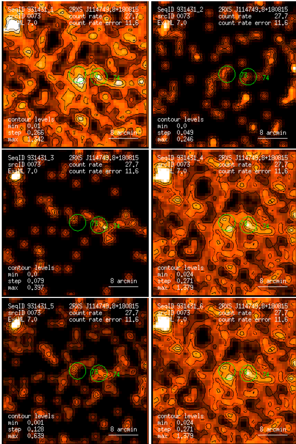
Figure 73: RASS 931431: detection 0073: band rate images, Gaussian filter: (1) PSPC channels 11 – 41, (2) 52 – 90, (3) 91 – 201, (4) 11 – 235, (5) 52 – 201, (6) 11 – 201. Broad band rates in counts/ks. Band rate contour levels in counts/ks/arcmin 2 .
