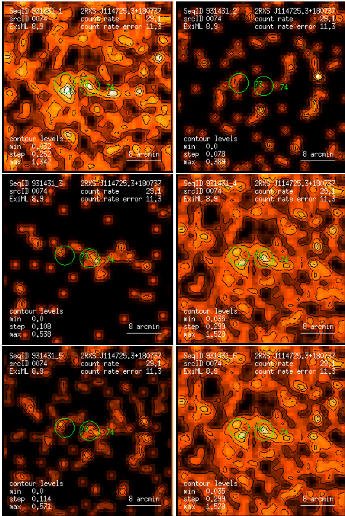
Figure 74: RASS 931431: detection 0074: band rate images, Gaussian filter: (1) PSPC channels 11 – 41, (2) 52 – 90, (3) 91 – 201, (4) 11 – 235, (5) 52 – 201, (6) 11 – 201. Broad band rates in counts/ks. Band rate contour levels in counts/ks/arcmin 2 .
