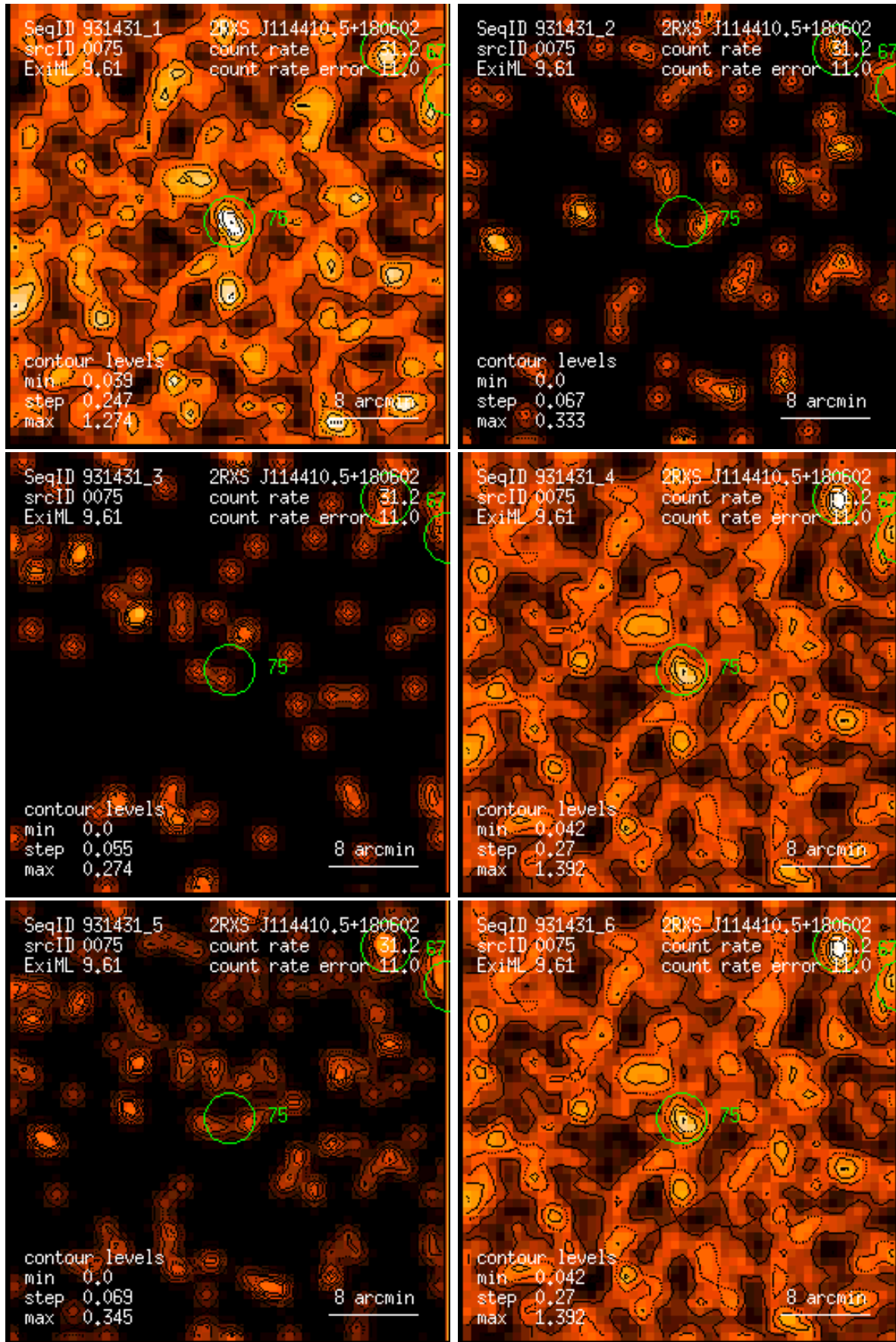
Figure 75: RASS 931431: detection 0075: band rate images, Gaussian filter: (1) PSPC channels 11 – 41, (2) 52 – 90, (3) 91 – 201, (4) 11 – 235, (5) 52 – 201, (6) 11 – 201. Broad band rates in counts/ks. Band rate contour levels in counts/ks/arcmin 2 .
