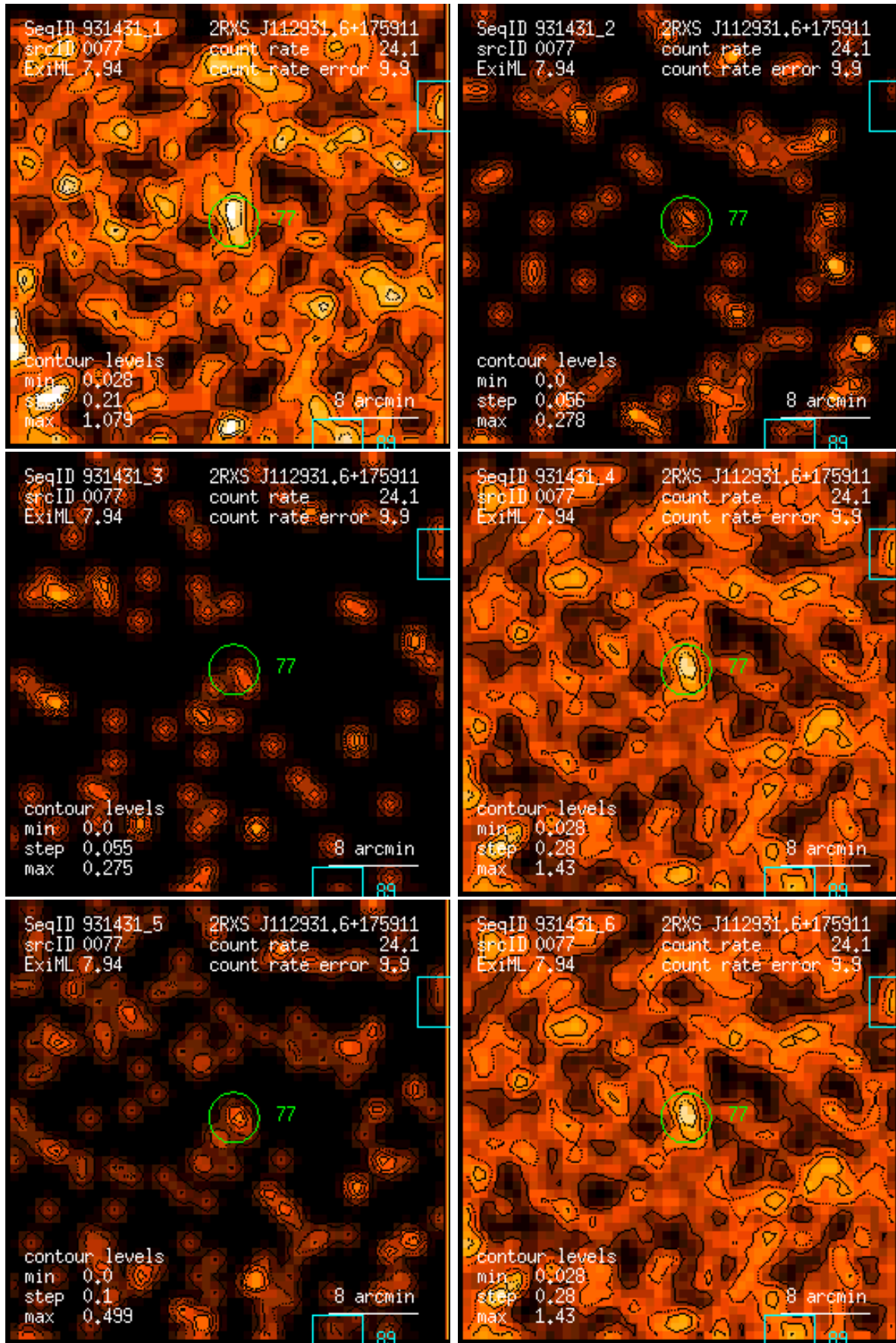
Figure 77: RASS 931431: detection 0077: band rate images, Gaussian filter: (1) PSPC channels 11 – 41, (2) 52 – 90, (3) 91 – 201, (4) 11 – 235, (5) 52 – 201, (6) 11 – 201. Broad band rates in counts/ks. Band rate contour levels in counts/ks/arcmin 2 .
