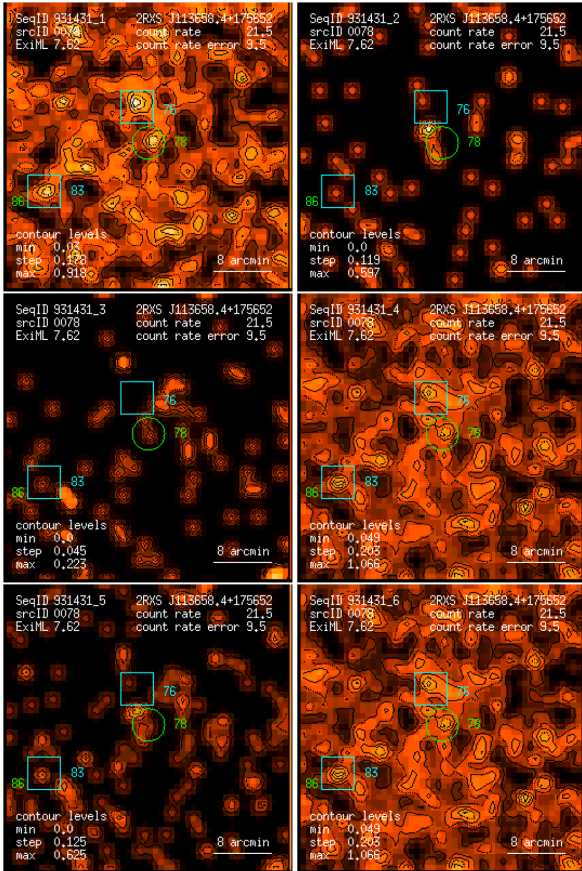
Figure 78: RASS 931431: detection 0078: band rate images, Gaussian filter: (1) PSPC channels 11 – 41, (2) 52 – 90, (3) 91 – 201, (4) 11 – 235, (5) 52 – 201, (6) 11 – 201. Broad band rates in counts/ks. Band rate contour levels in counts/ks/arcmin 2 .
