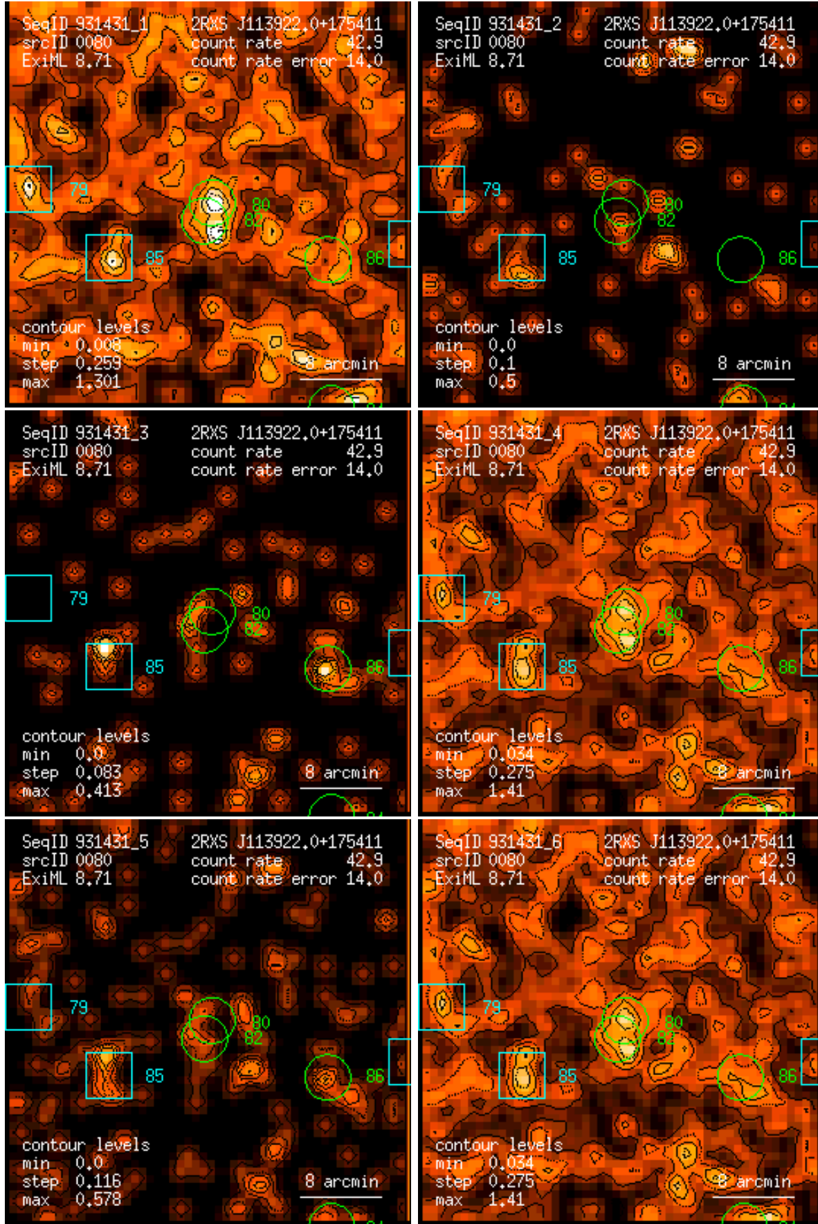
Figure 80: RASS 931431: detection 0080: band rate images, Gaussian filter: (1) PSPC channels 11 – 41, (2) 52 – 90, (3) 91 – 201, (4) 11 – 235, (5) 52 – 201, (6) 11 – 201. Broad band rates in counts/ks. Band rate contour levels in counts/ks/arcmin 2 .
