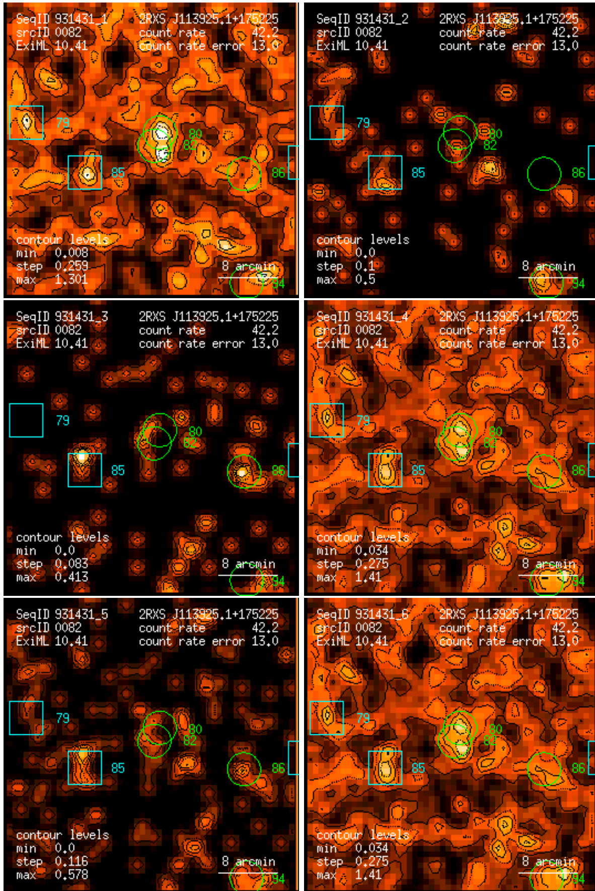
Figure 82: RASS 931431: detection 0082: band rate images, Gaussian filter: (1) PSPC channels 11 – 41, (2) 52 – 90, (3) 91 – 201, (4) 11 – 235, (5) 52 – 201, (6) 11 – 201. Broad band rates in counts/ks. Band rate contour levels in counts/ks/arcmin 2 .
