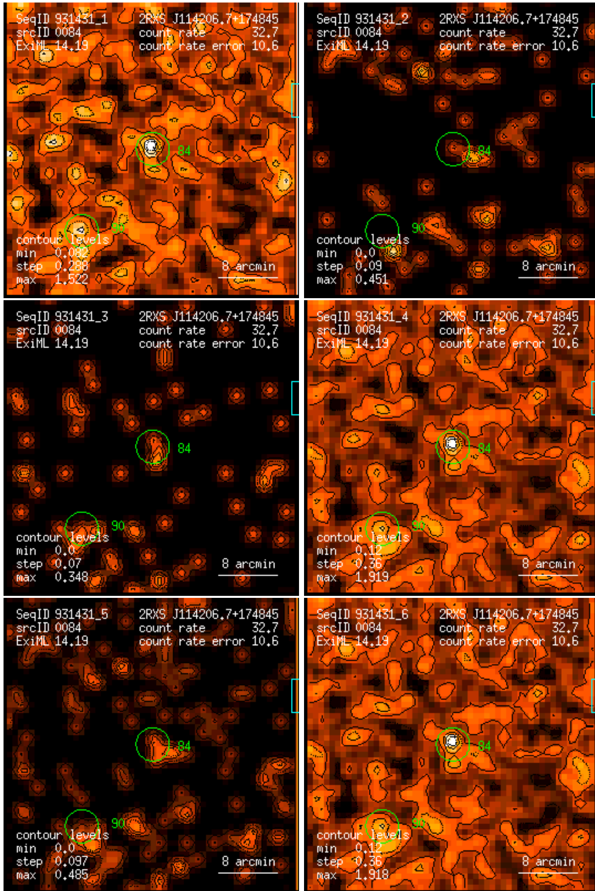
Figure 84: RASS 931431: detection 0084: band rate images, Gaussian filter: (1) PSPC channels 11 – 41, (2) 52 – 90, (3) 91 – 201, (4) 11 – 235, (5) 52 – 201, (6) 11 – 201. Broad band rates in counts/ks. Band rate contour levels in counts/ks/arcmin 2 .
