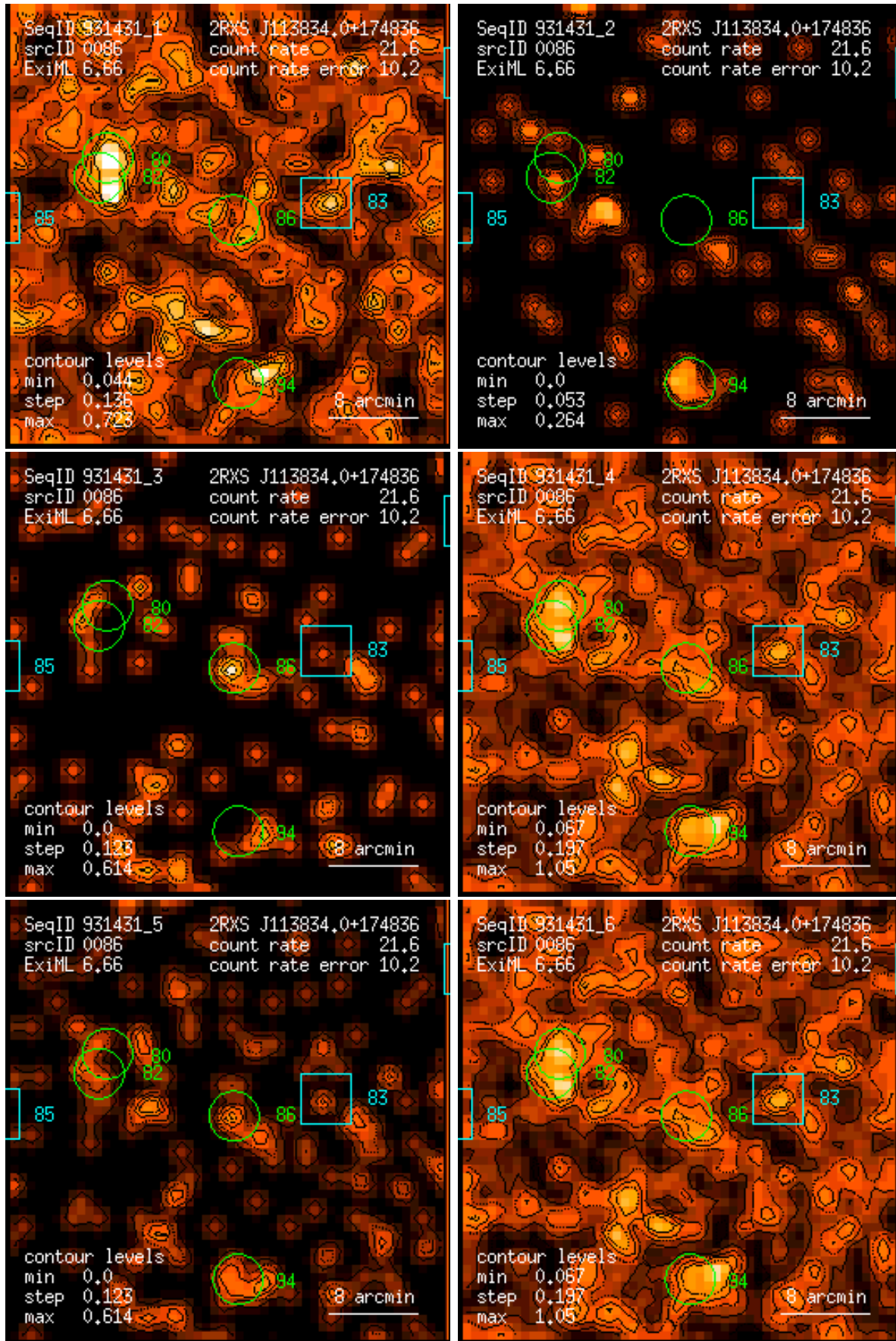
Figure 86: RASS 931431: detection 0086: band rate images, Gaussian filter: (1) PSPC channels 11 – 41, (2) 52 – 90, (3) 91 – 201, (4) 11 – 235, (5) 52 – 201, (6) 11 – 201. Broad band rates in counts/ks. Band rate contour levels in counts/ks/arcmin 2 .
