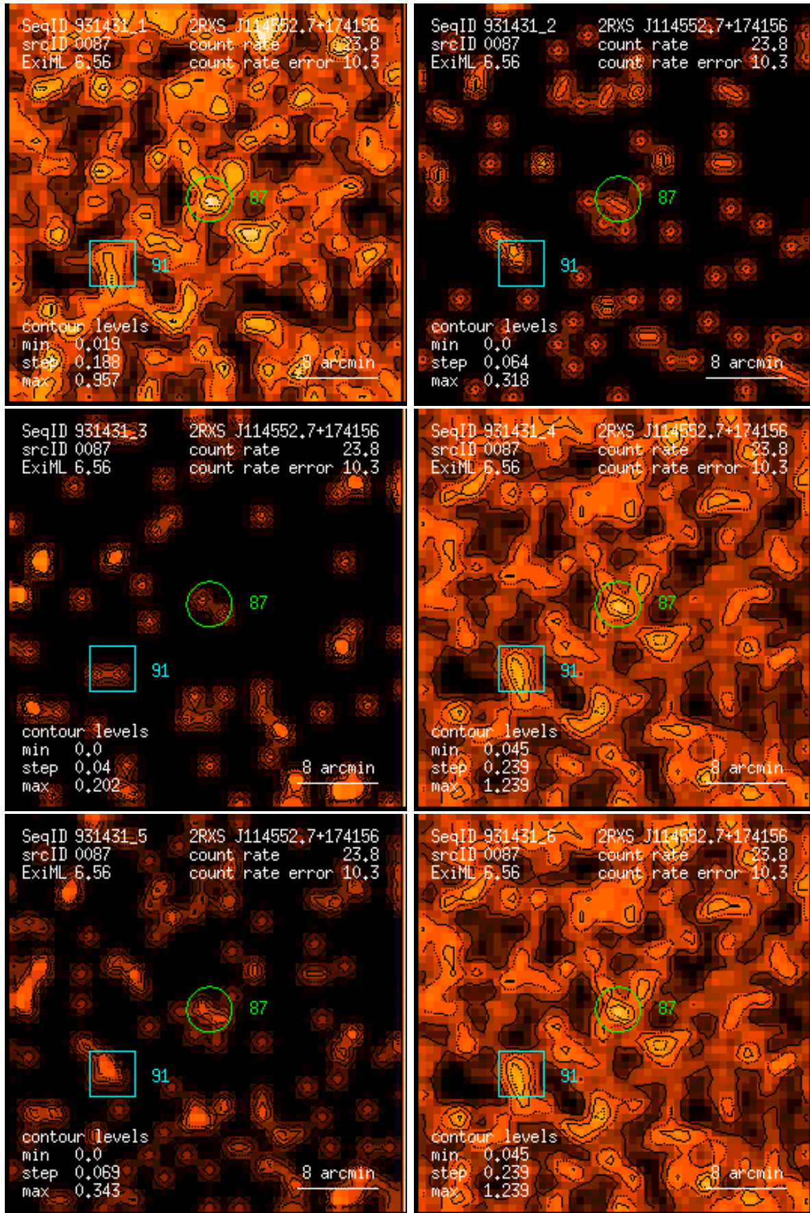
Figure 87: RASS 931431: detection 0087: band rate images, Gaussian filter: (1) PSPC channels 11 – 41, (2) 52 – 90, (3) 91 – 201, (4) 11 – 235, (5) 52 – 201, (6) 11 – 201. Broad band rates in counts/ks. Band rate contour levels in counts/ks/arcmin 2 .
