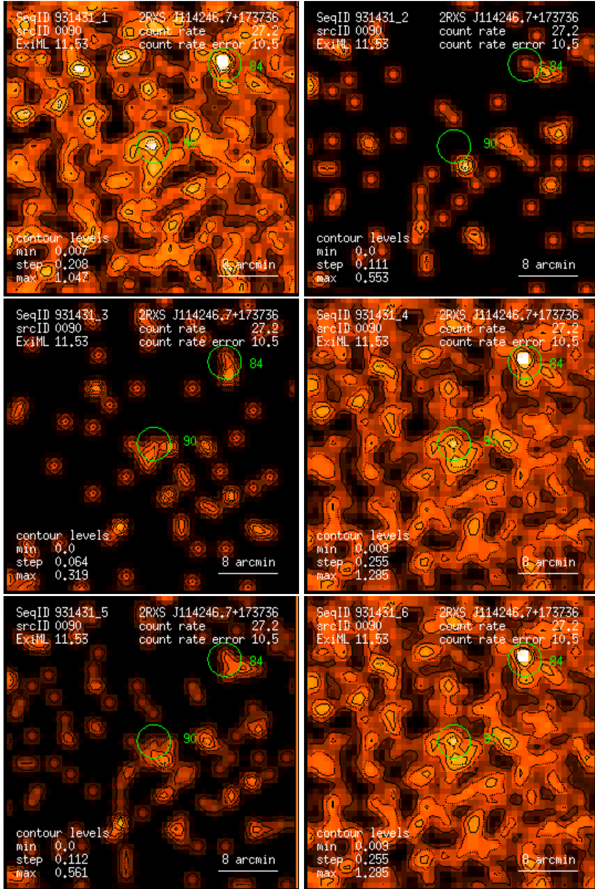
Figure 90: RASS 931431: detection 0090: band rate images, Gaussian filter: (1) PSPC channels 11 – 41, (2) 52 – 90, (3) 91 – 201, (4) 11 – 235, (5) 52 – 201, (6) 11 – 201. Broad band rates in counts/ks. Band rate contour levels in counts/ks/arcmin 2 .
