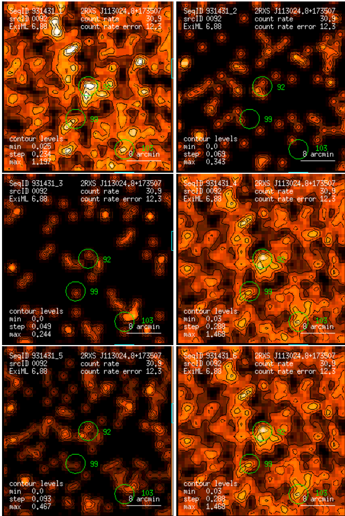
Figure 92: RASS 931431: detection 0092: band rate images, Gaussian filter: (1) PSPC channels 11 – 41, (2) 52 – 90, (3) 91 – 201, (4) 11 – 235, (5) 52 – 201, (6) 11 – 201. Broad band rates in counts/ks. Band rate contour levels in counts/ks/arcmin 2 .
