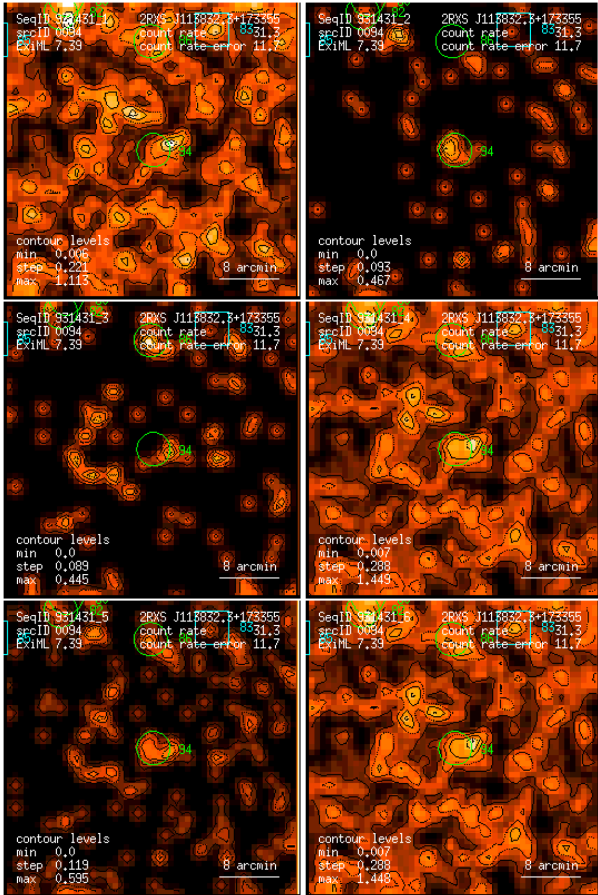
Figure 94: RASS 931431: detection 0094: band rate images, Gaussian filter: (1) PSPC channels 11 – 41, (2) 52 – 90, (3) 91 – 201, (4) 11 – 235, (5) 52 – 201, (6) 11 – 201. Broad band rates in counts/ks. Band rate contour levels in counts/ks/arcmin 2 .
