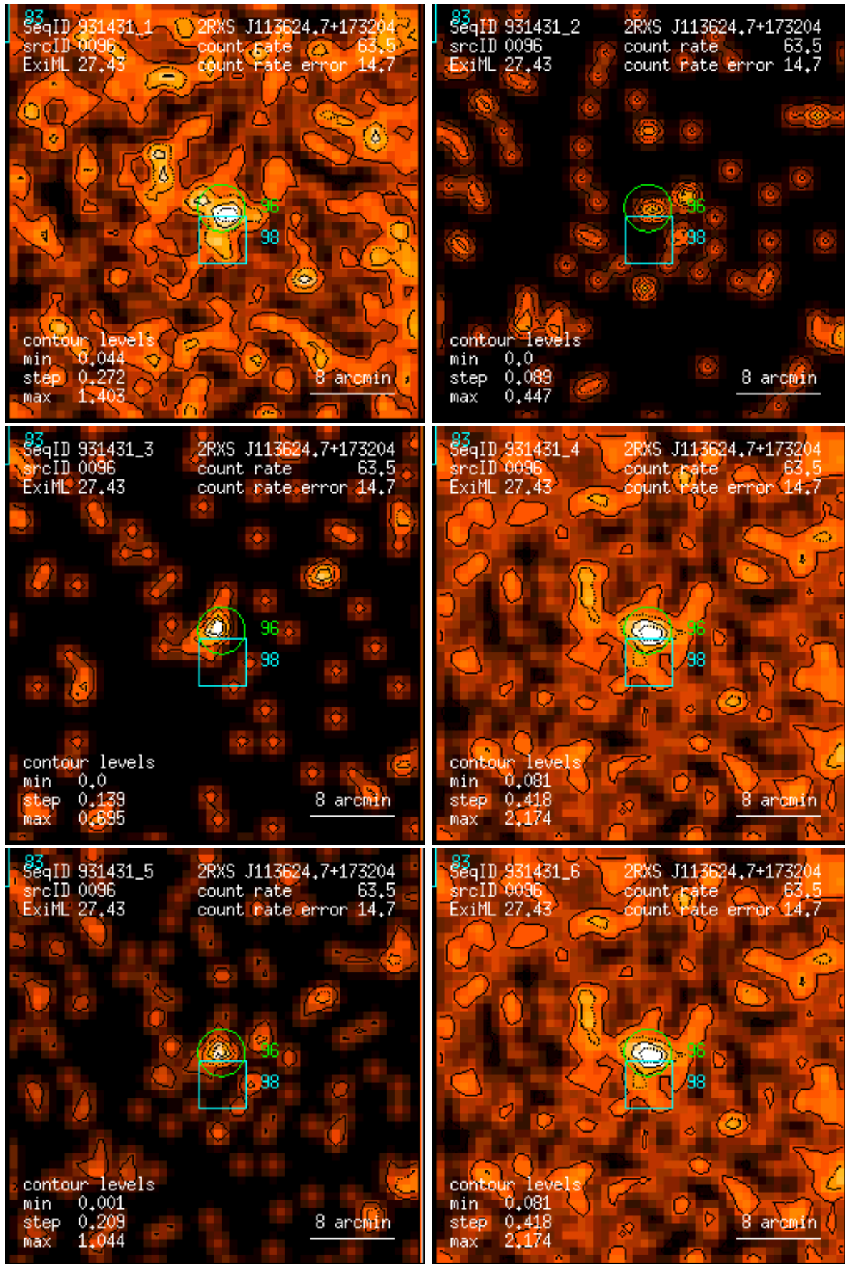
Figure 96: RASS 931431: detection 0096: band rate images, Gaussian filter: (1) PSPC channels 11 – 41, (2) 52 – 90, (3) 91 – 201, (4) 11 – 235, (5) 52 – 201, (6) 11 – 201. Broad band rates in counts/ks. Band rate contour levels in counts/ks/arcmin 2 .
